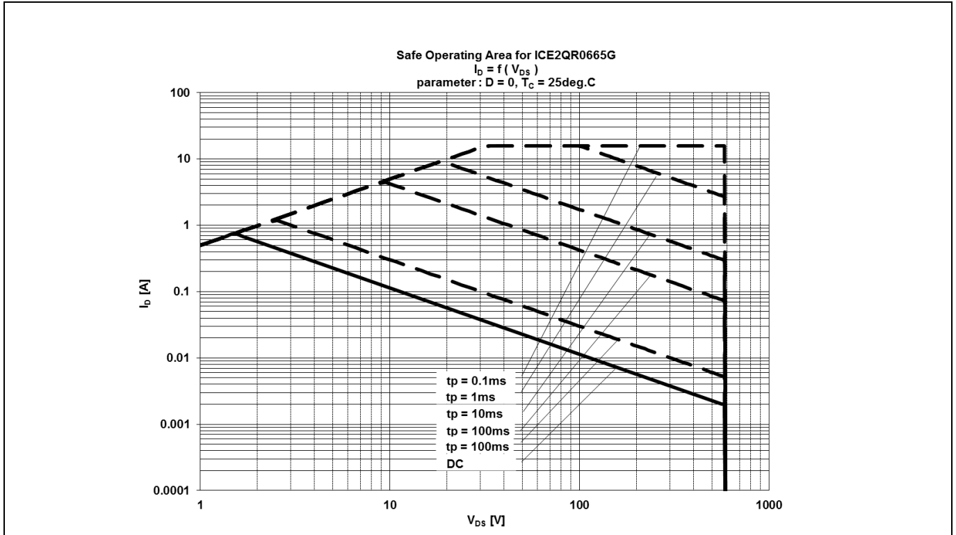
Figure 10 Safe Operating Area (SOA) curve for ICE2QR0665G
