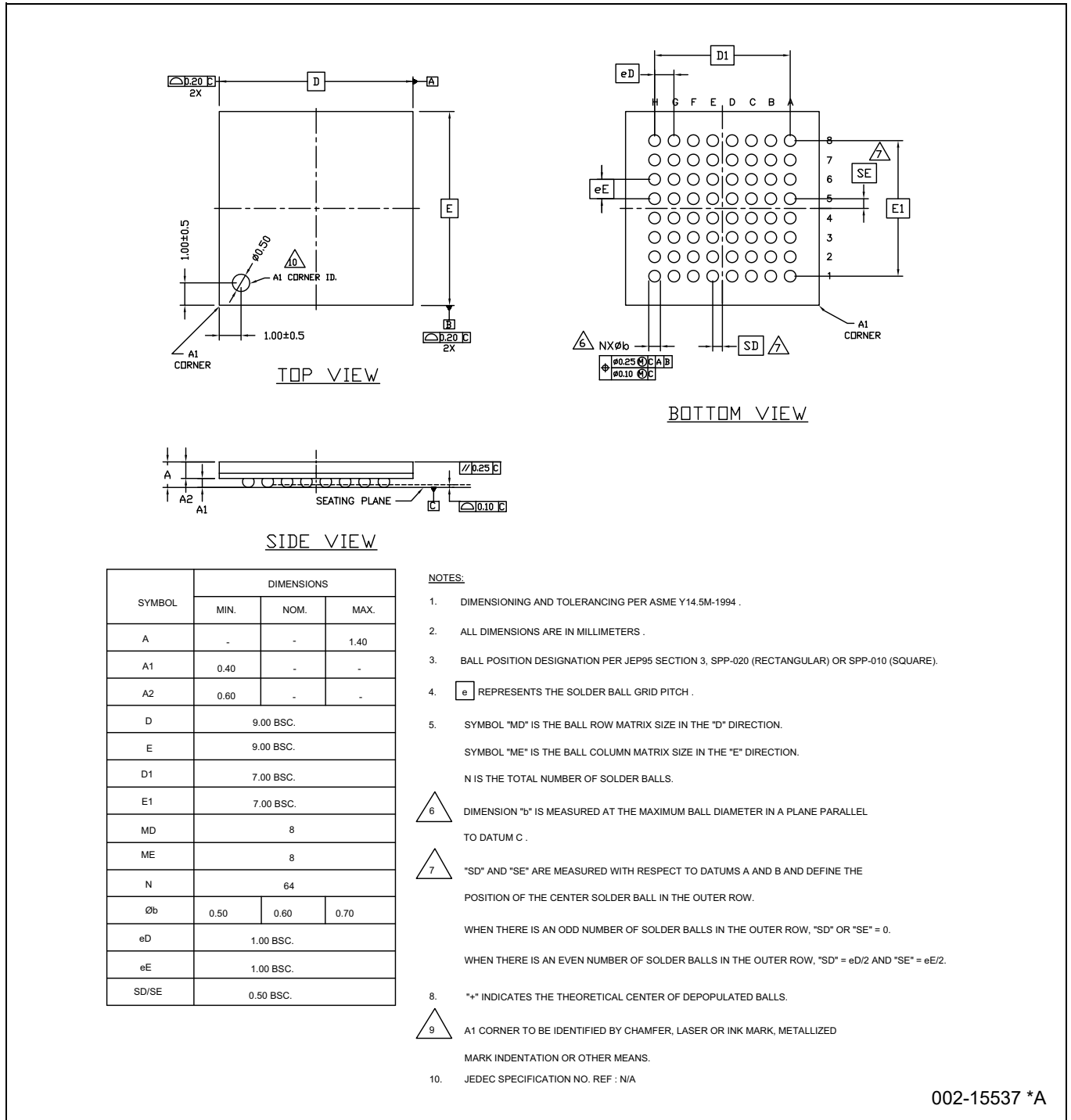
Figure 37 64-ball FBGA 9.0 x 9.0 x 1.4 mm LAE064, package outline (PG-LFBGA-64)
