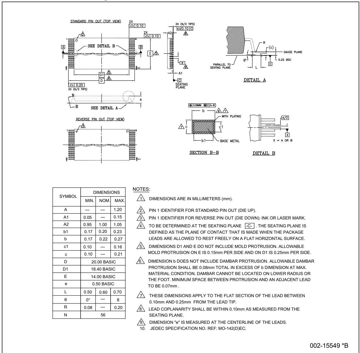
Figure 35 56-lead TSOP 18.4 x 14.0 x 1.2 mm TS056/TSR056, package outline (PG-TSOP-56)
