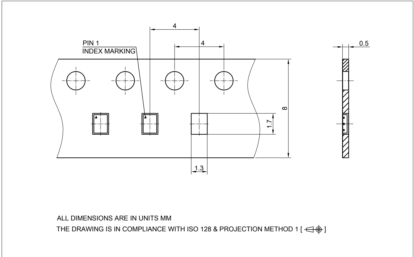
Figure 21 TSNP-6 packaging
