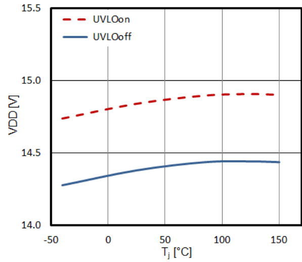
4. Undervoltage lockout threshold (1EDN9550) vs temperature
