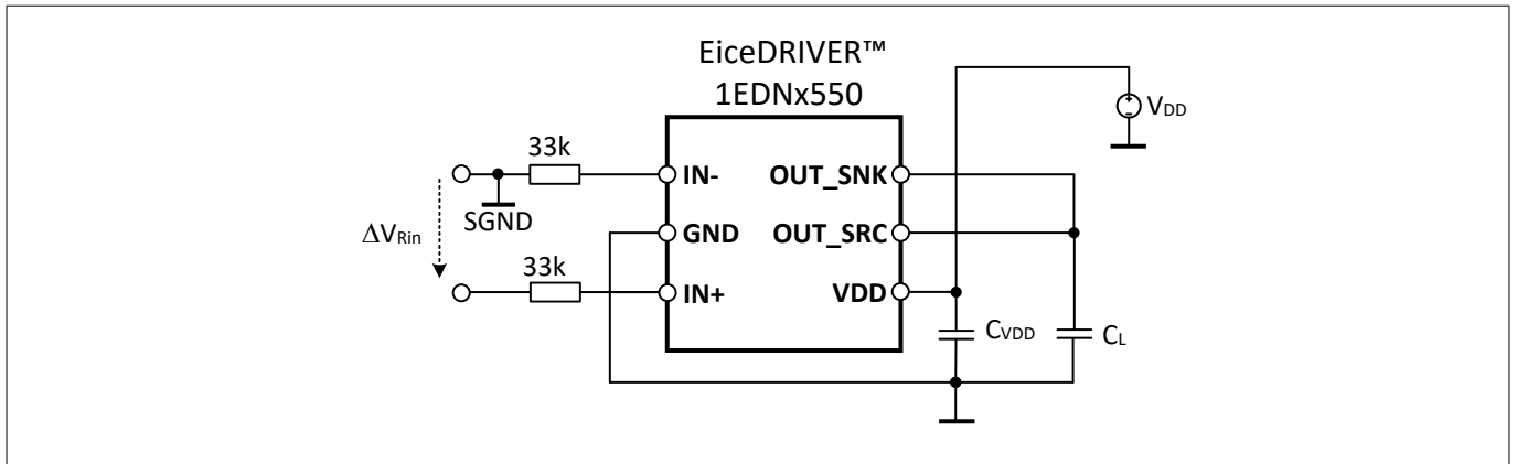
Figure 5 Test circuit
