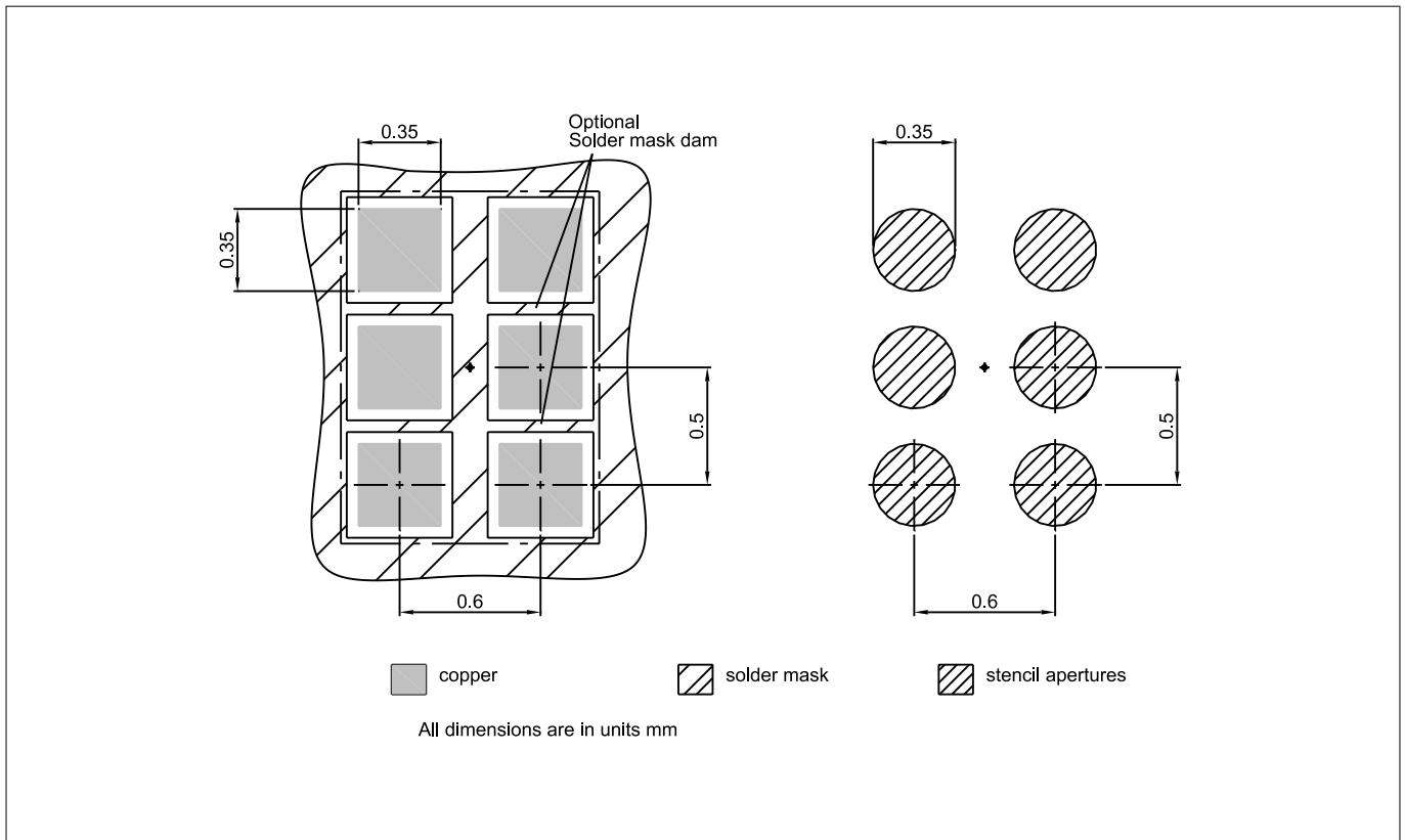
Figure 20 TSNP-6 footprint
