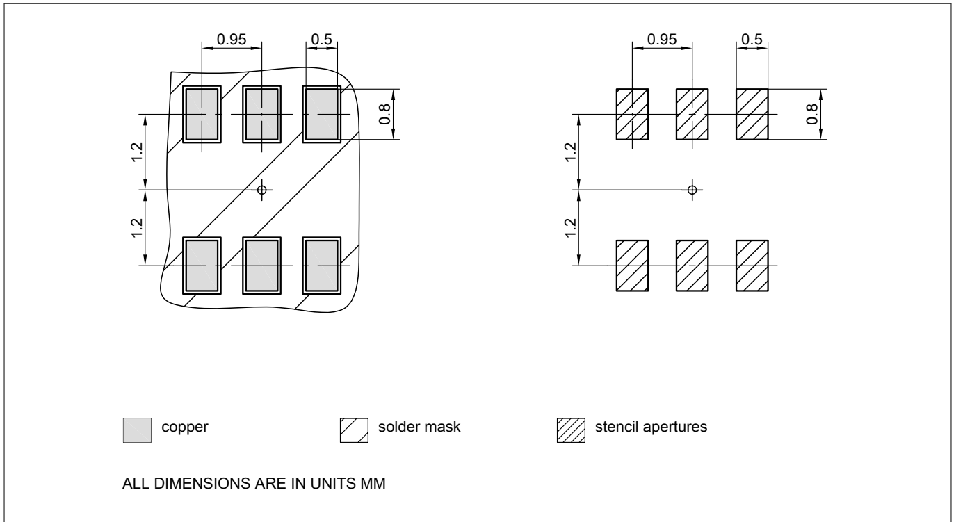
Figure 16 PG-SOT23-6 footprint
