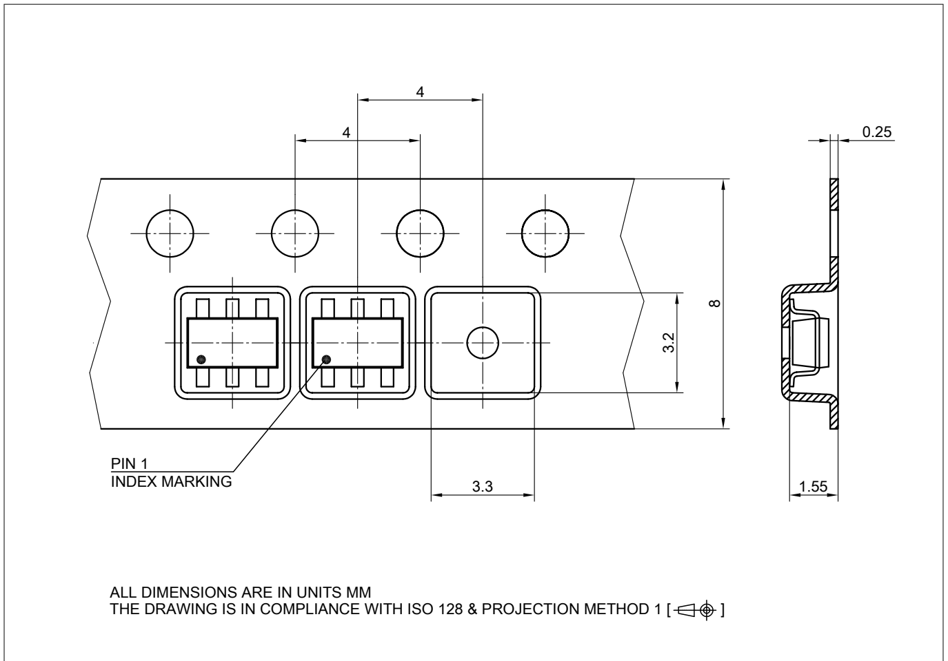
Figure 17 PG-SOT23-6 packaging
