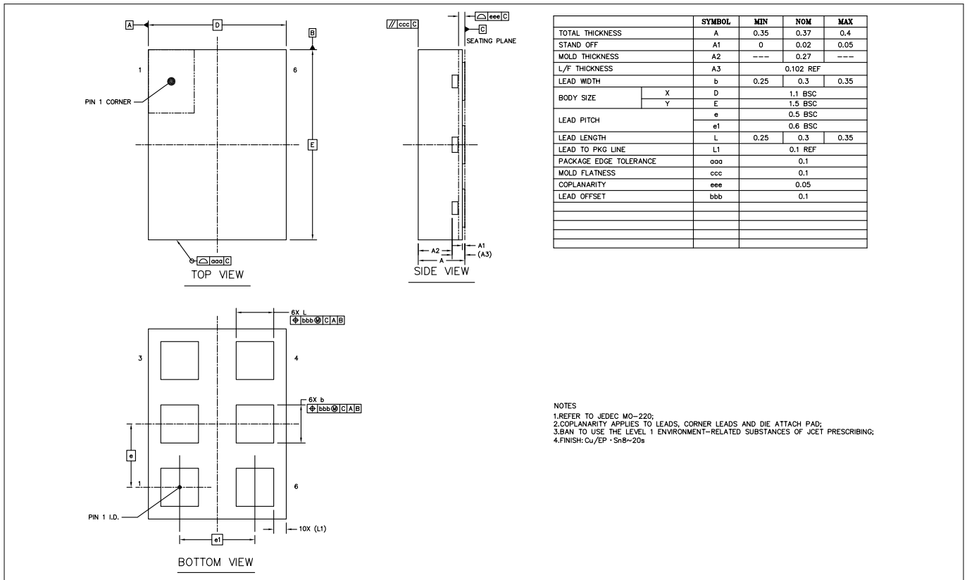
Figure 19 TSNP-6 outline
