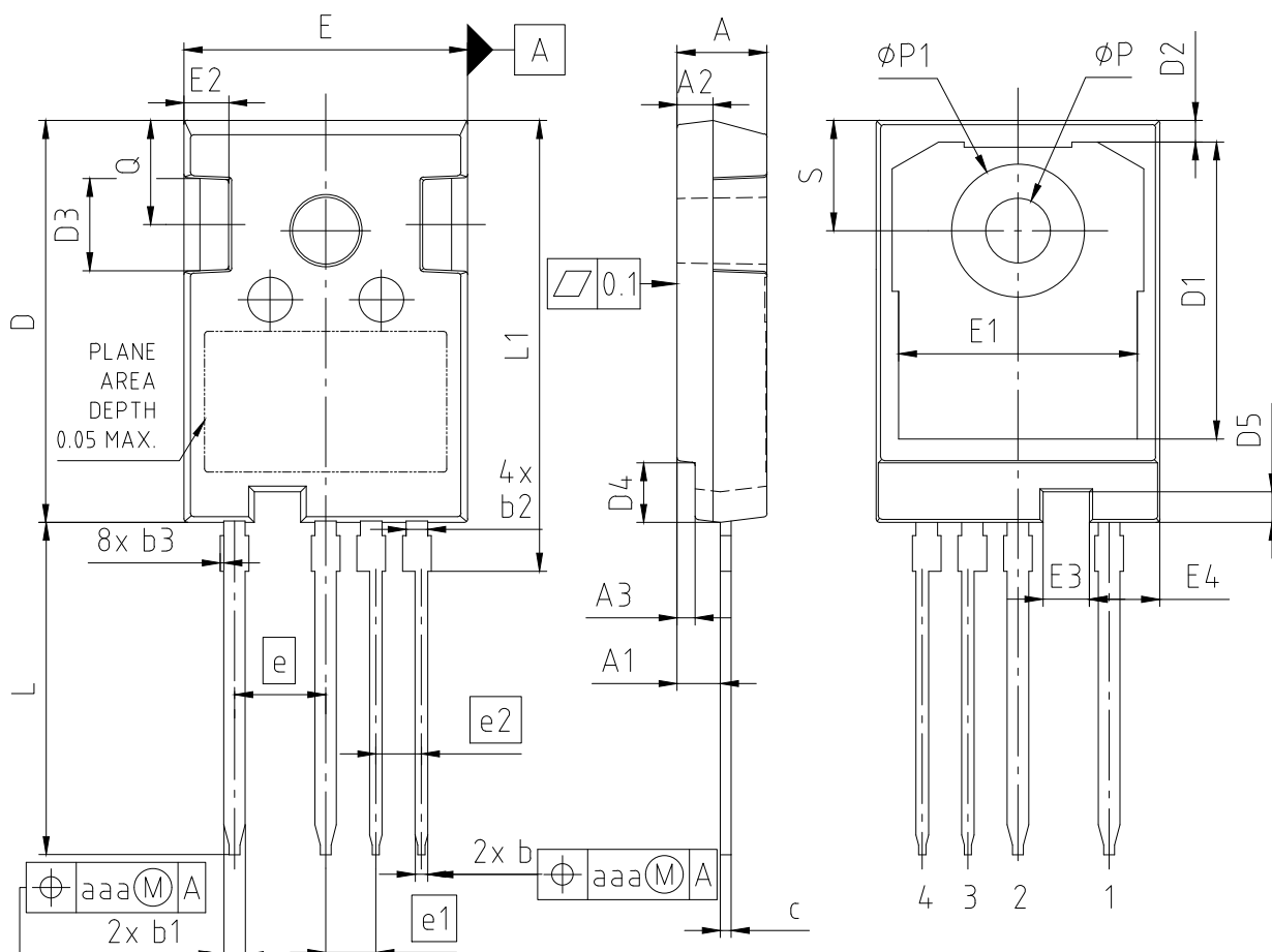
PG-TO247-4-STD-NT6.7
