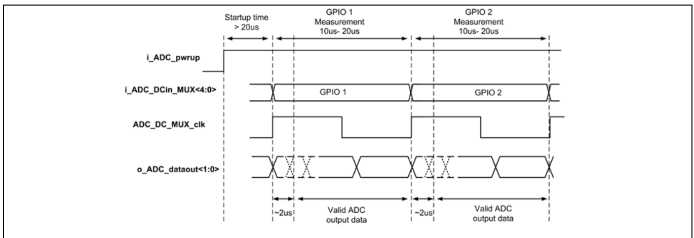
Figure 2 Mux clcking and timing diagram of ADC
