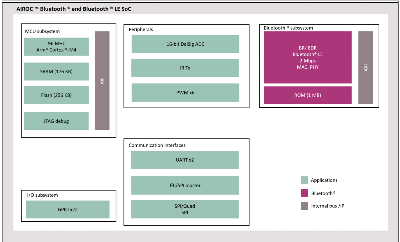
Figure 1 Block diagram of CYW20819/CYW20820 Bluetooth® SoC
