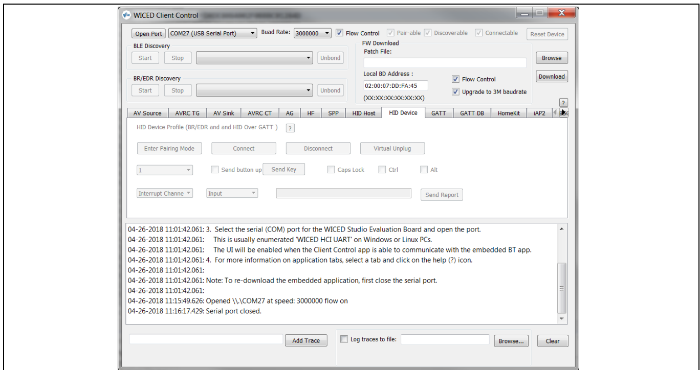
Figure 8 ClientControl window
