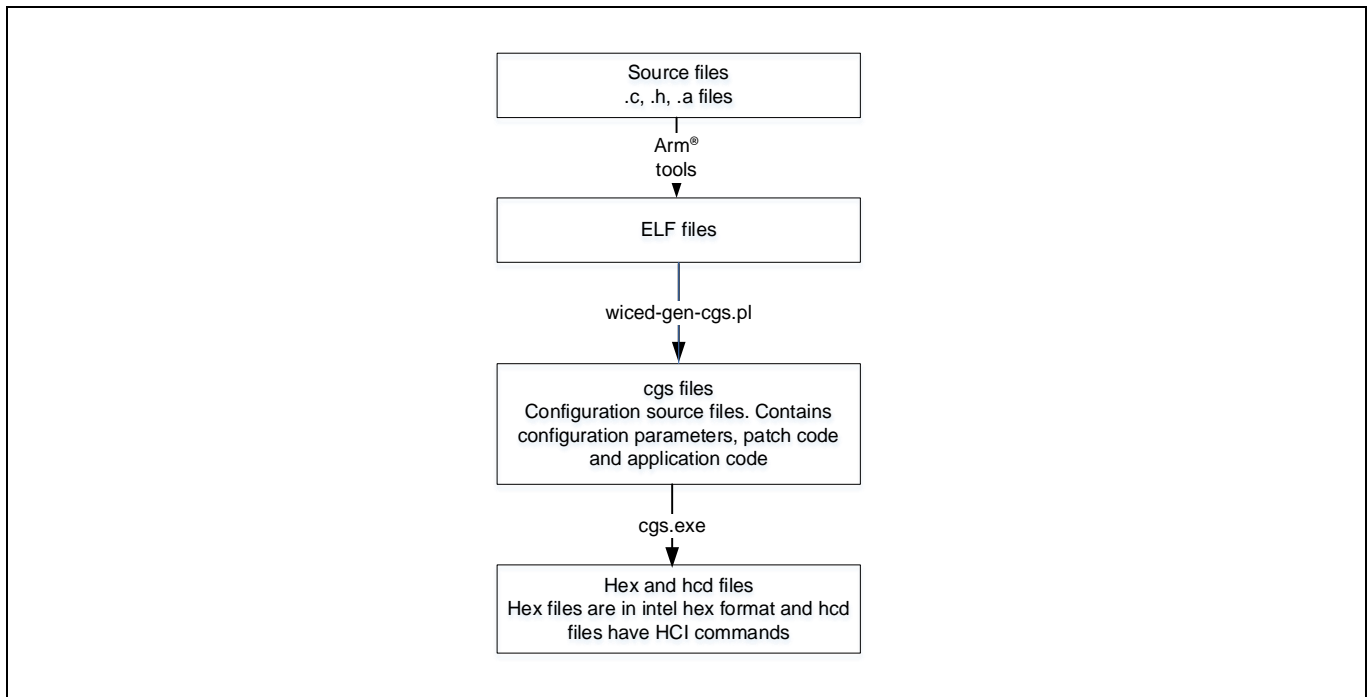
Figure 7 File formats
