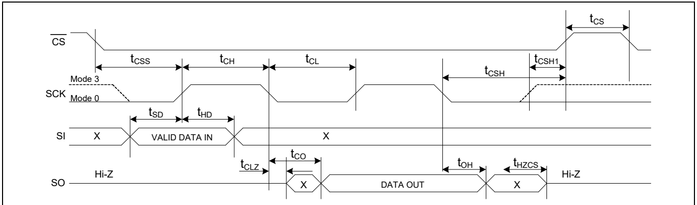
Figure 20 Synchronous data timing (Mode 0 and Mode 3)
