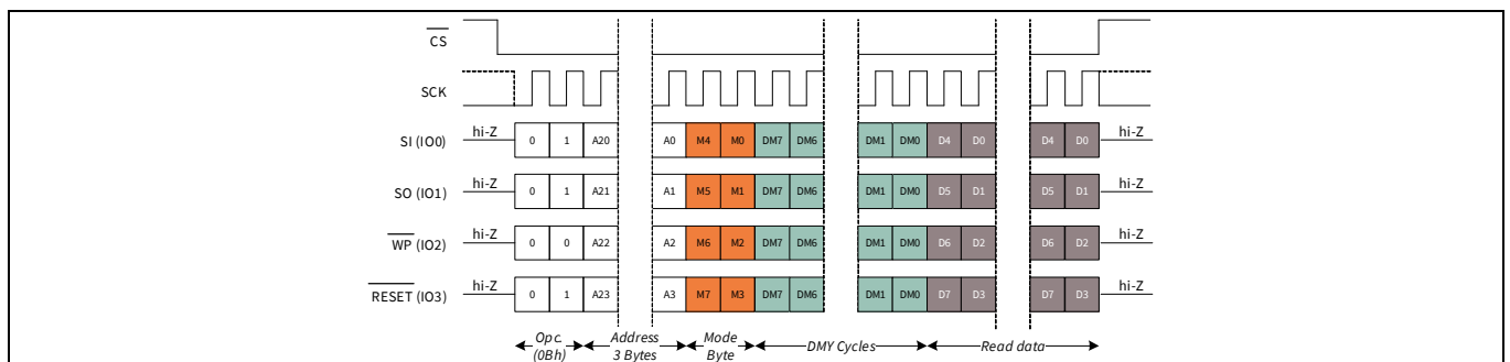
Figure 57 FAST_READ in QPI mode
