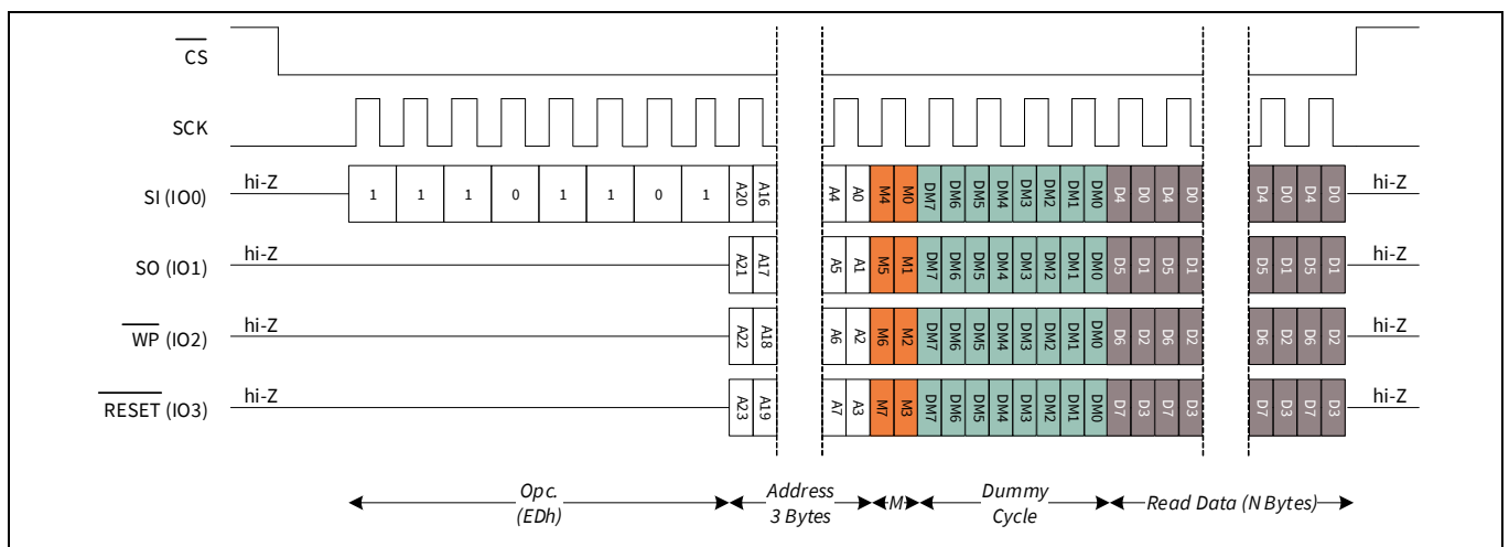
Figure 65 Quad I/O Read in DDR (DDRQIOR) – In Extended SPI mode
