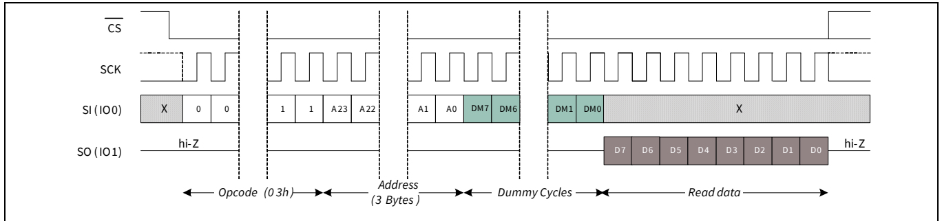
Figure 52 READ in SPI mode
