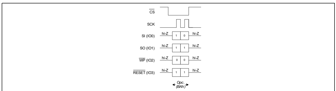
Figure 106 Hibernate mode operation in QPI mode
