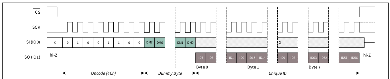
Figure 91 Read Unique ID in SPI mode
