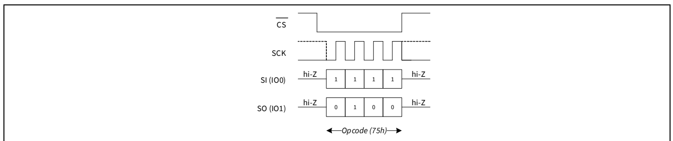
Figure 83 CRC Suspend (EPCS) in DPI mode
