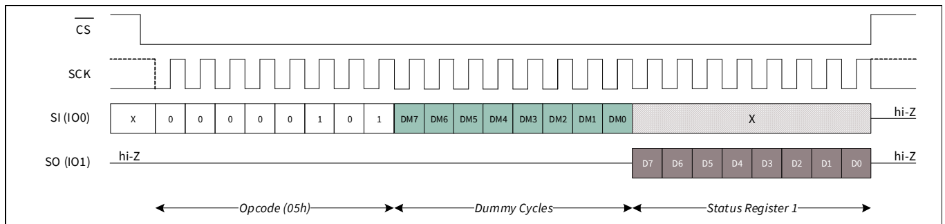
Figure 15 Read SR1 (RDSR1) in SPI mode
