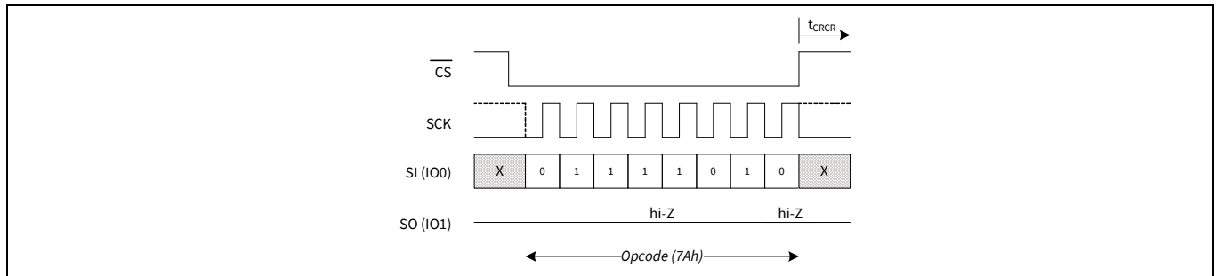
Figure 85 CRC Resume (EPCR) in SPI mode
