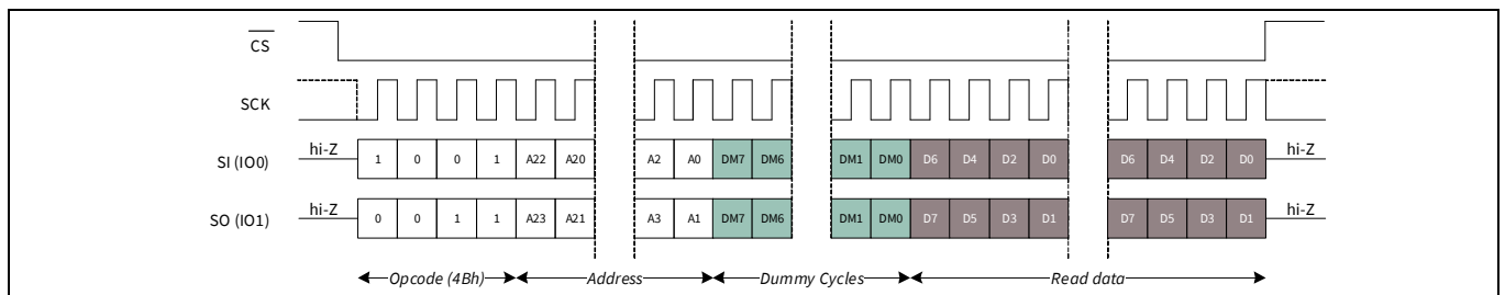
Figure 71 Special Sector Read (SSRD) in DPI mode
