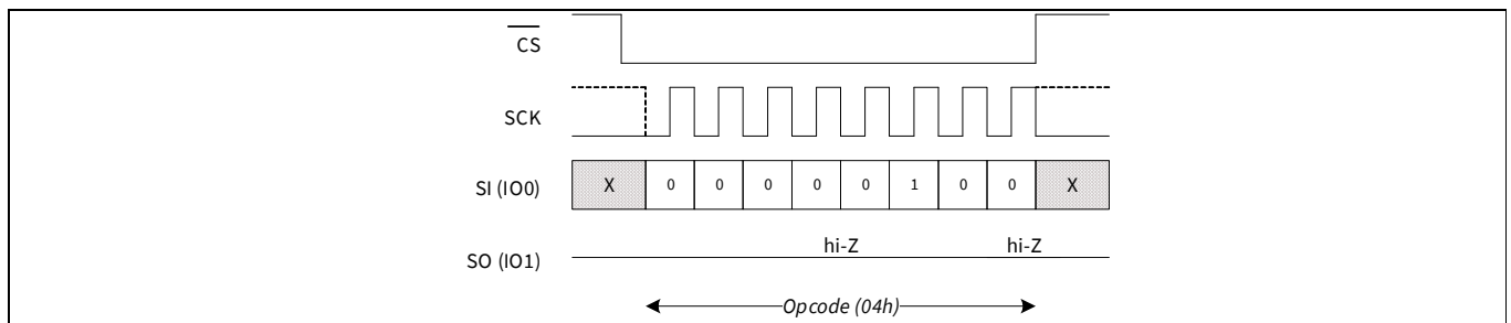
Figure 9 WRDI bus configuration in SPI mode
