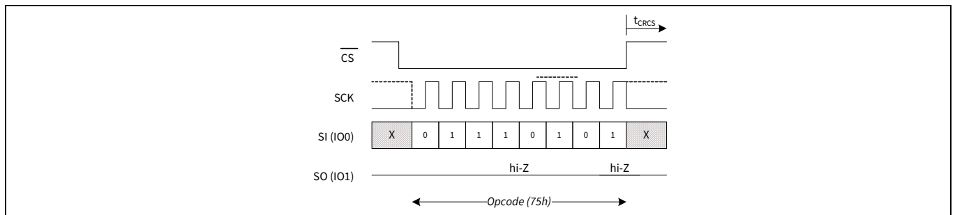
Figure 82 CRC Suspend (EPCS) in SPI Mode
