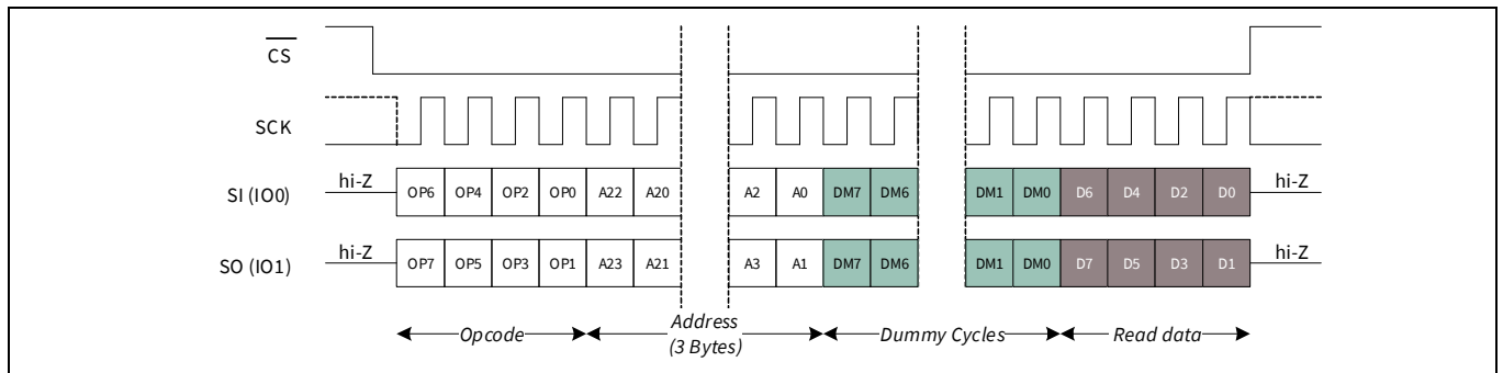
Figure 37 Read Any Register (RDAR) in DPI mode
