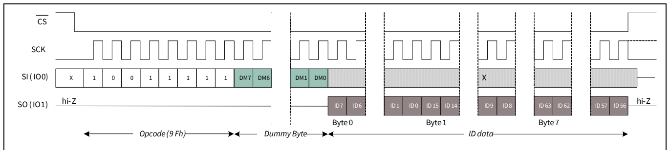
Figure 88 Read Device ID (RDID) in SPI mode
