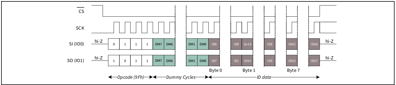
Figure 89 Read Device ID (RDID) in DPI mode
