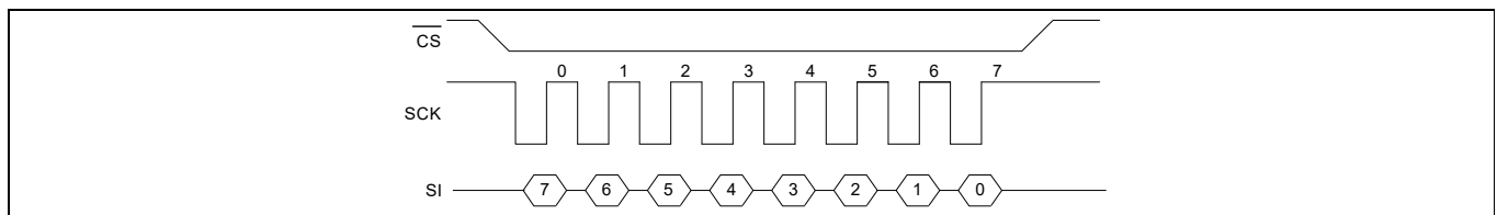
Figure 5 SPI Mode 3
