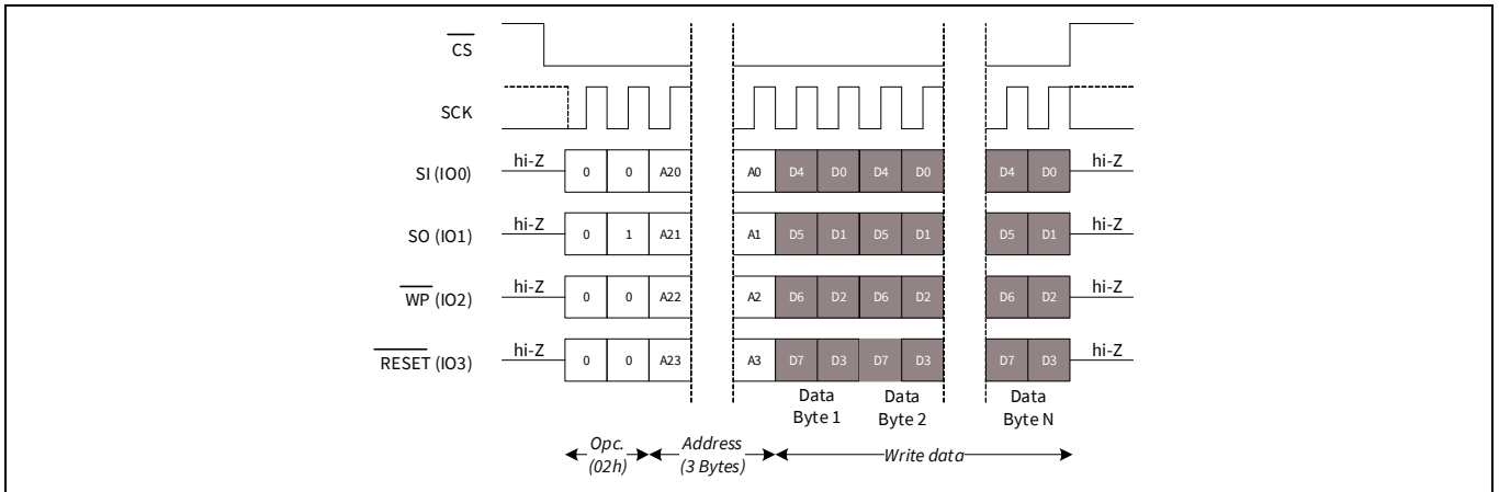
Figure 41 Memory Write (WRITE) in QPI mode
