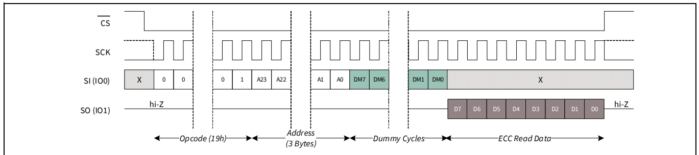
Figure 73 ECC Read (ECCRD) in SPI mode
