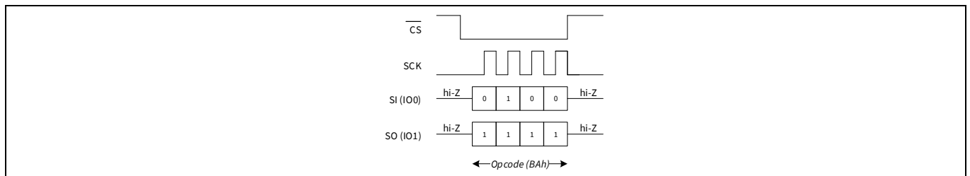
Figure 105 Hibernate mode operation in DPI mode
