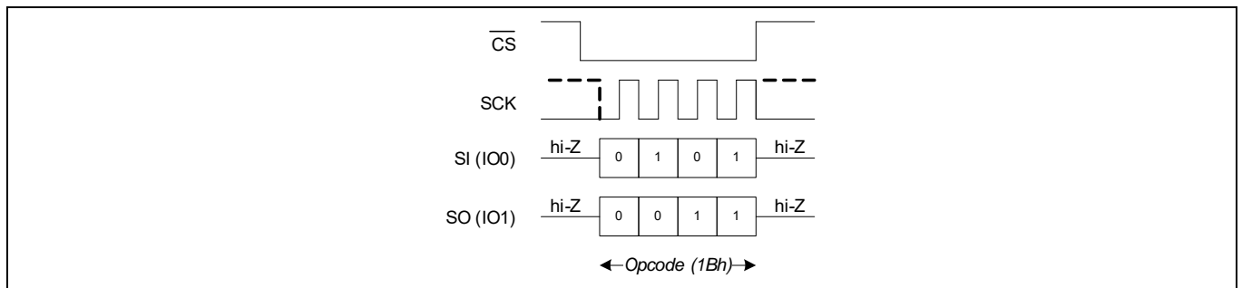
Figure 77 Clear ECC (CLECC) in DPI mode
