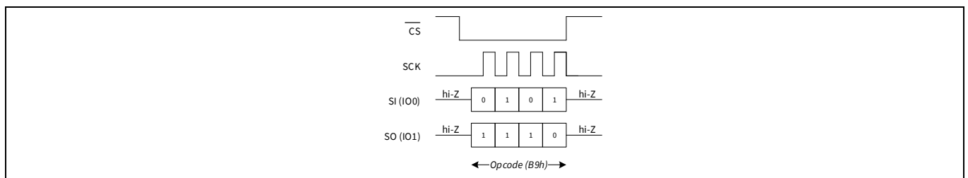
Figure 101 Deep power-down mode operation in DPI mode
