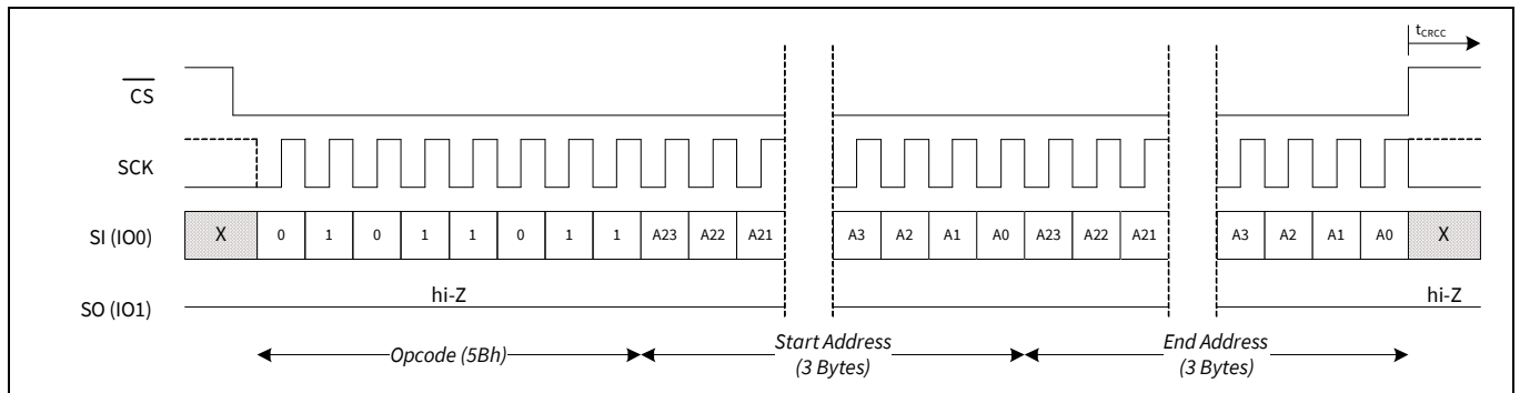
Figure 79 CRC Calculation (CRCC) in SPI mode
