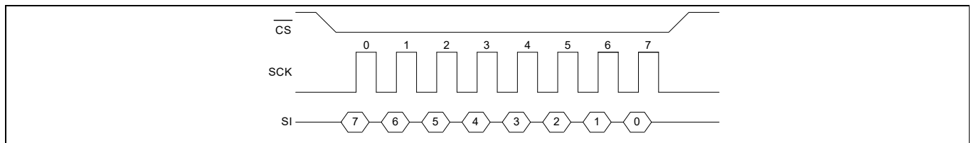
Figure 4 SPI Mode 0
