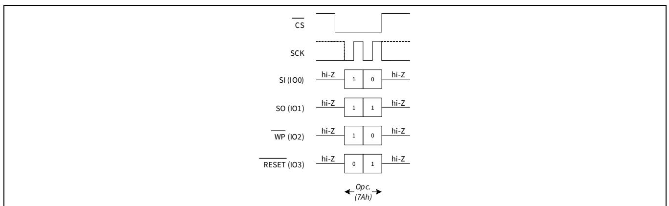
Figure 87 CRC Resume (EPCR) in QPI Mode
