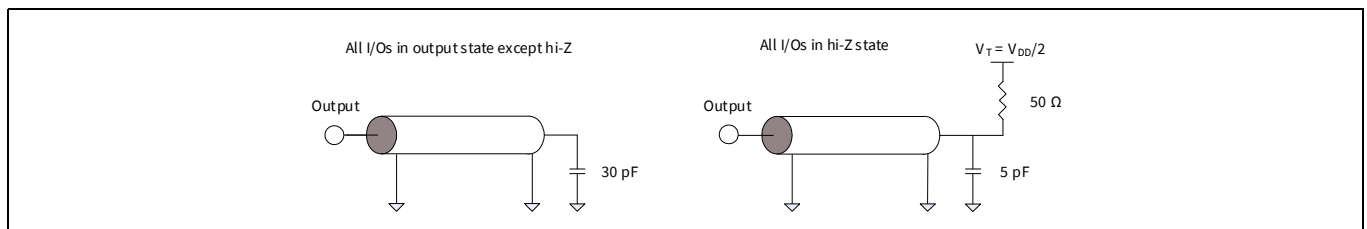
Figure 113 AC test loads
