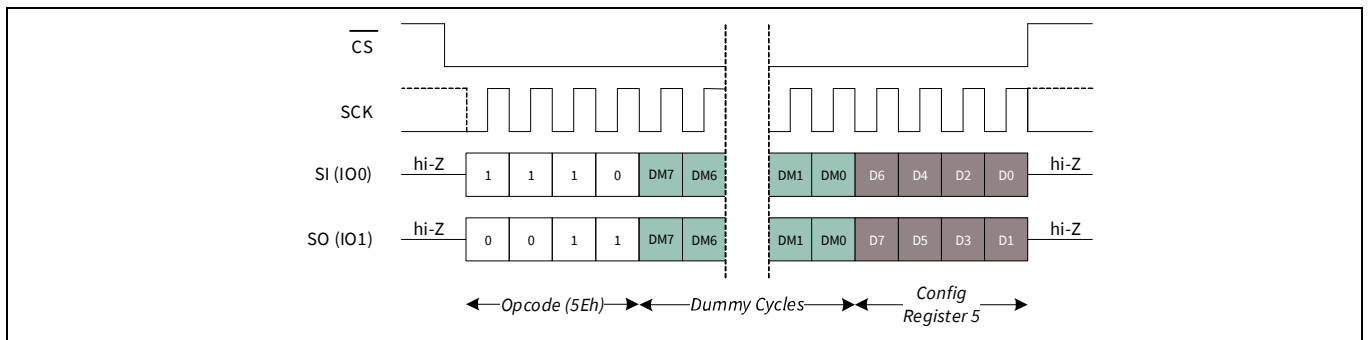
Figure 31 Read CR5 (RDCR5) in DPI mode
