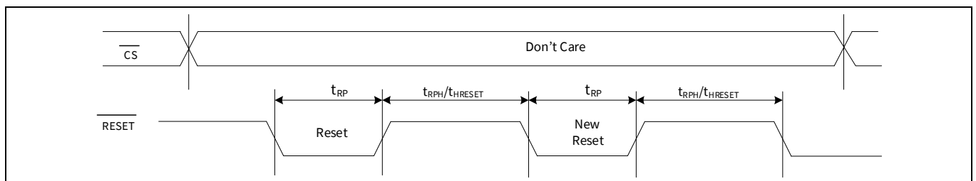
Figure 111 \overline{\text{RESET}} timing - QUAD clear (CR1[1] = ‘0’) and QPI disabled (CR2[6] = ‘0’)
