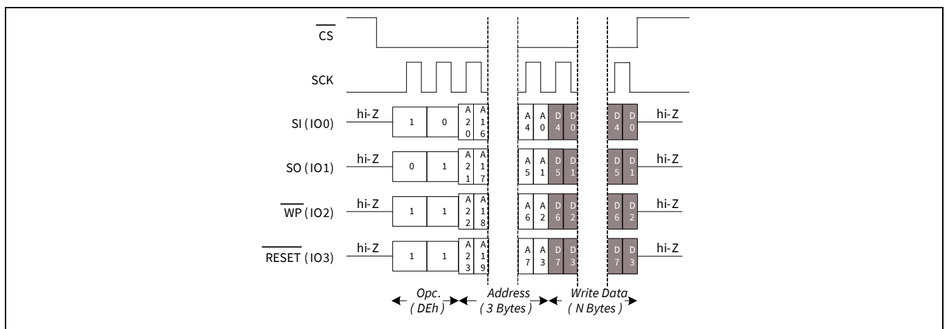
Figure 42 DDR Write (DDRWRITE) in QPI mode
