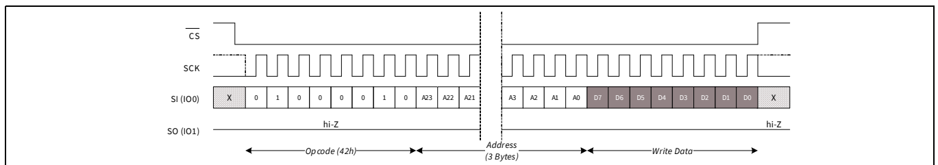
Figure 67 Special Sector Write (SSWR) in SPI Mode (WREN is not shown)
