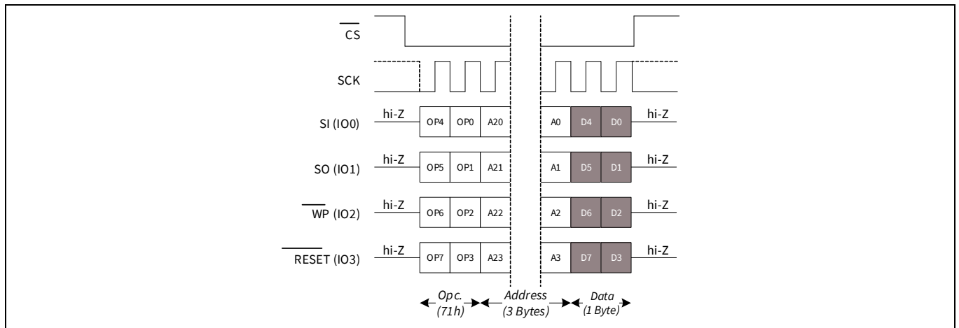
Figure 35 Write Any Register (WRAR) in QPI mode
