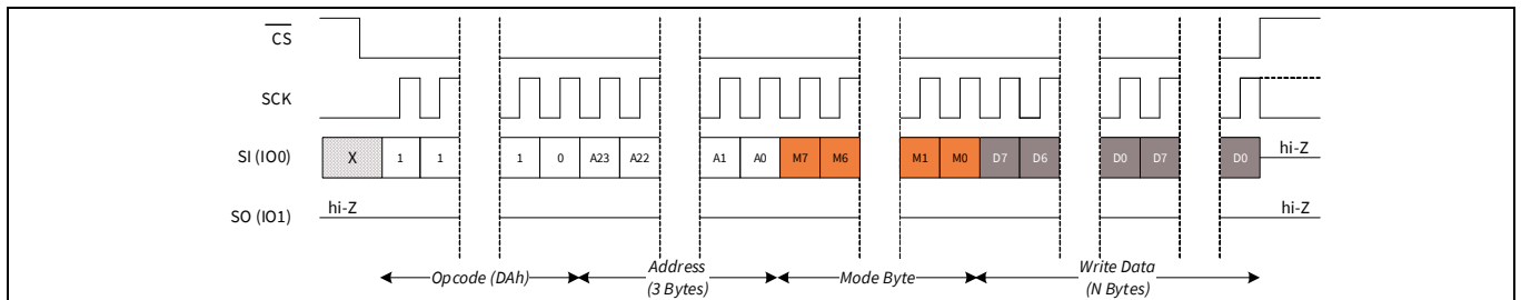
Figure 43 Fast Write (FAST_WRITE) in SPI mode
