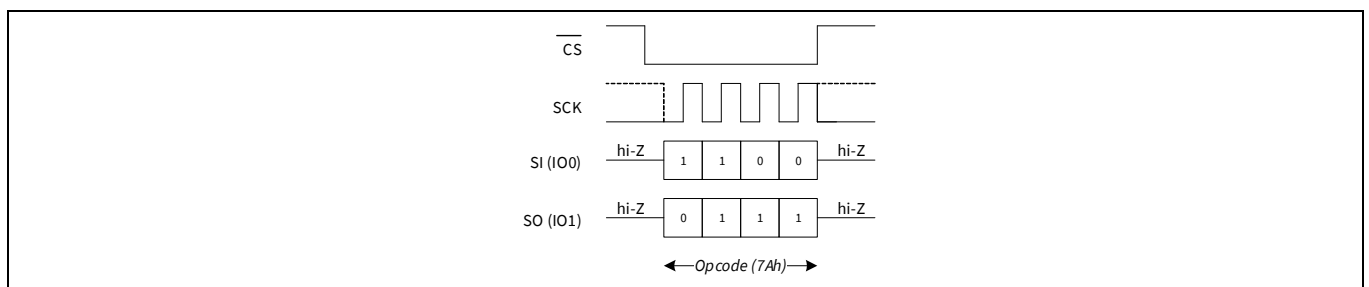
Figure 86 CRC Resume (EPCR) in DPI mode
