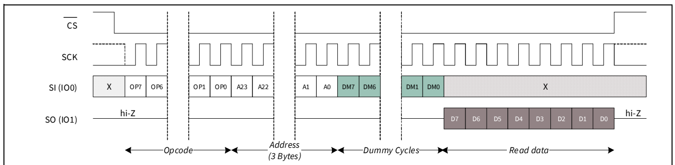
Figure 36 Read Any Register (RDAR) in SPI mode
