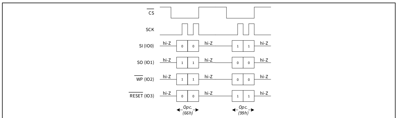
Figure 109 Software Reset timing in QPI mode
