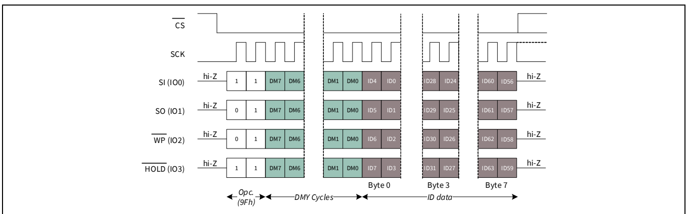
Figure 90 Read Device ID (RDID) in QPI mode
