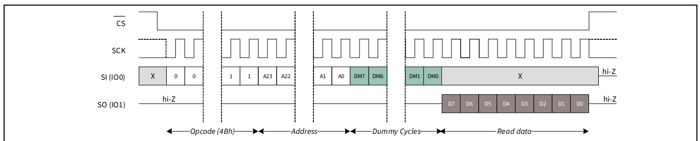
Figure 70 Special Sector Read (SSRD) in SPI mode
