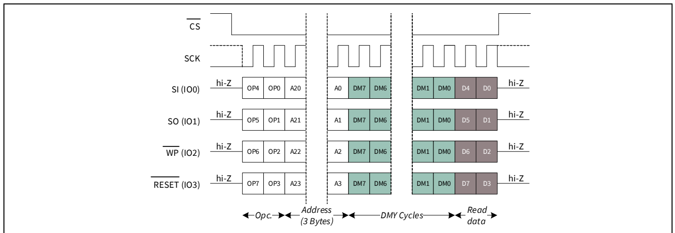
Figure 38 Read Any Register (RDAR) in QPI mode
