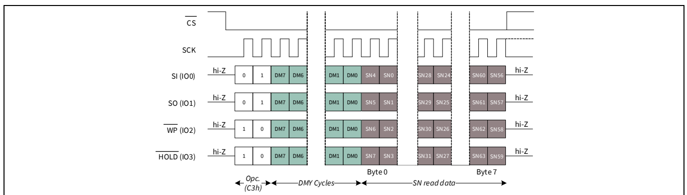
Figure 99 Read Serial Number (RDSN) in QPI mode
