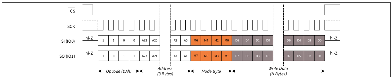
Figure 44 Fast Write (FAST_WRITE) in DPI mode
