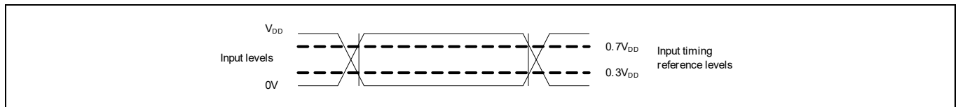
Figure 114 AC timing input voltage reference levels
