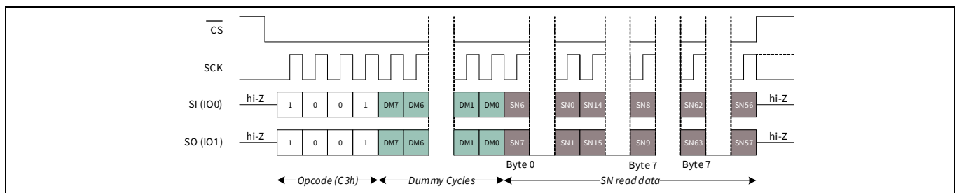
Figure 98 Read Serial Number (RDSN) in DPI mode
