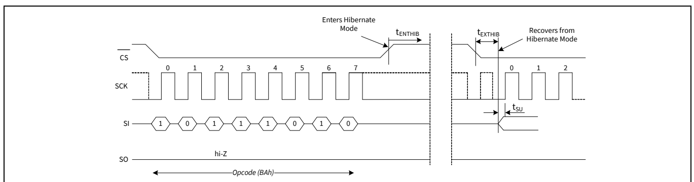
Figure 104 Hibernate mode operation in SPI mode
