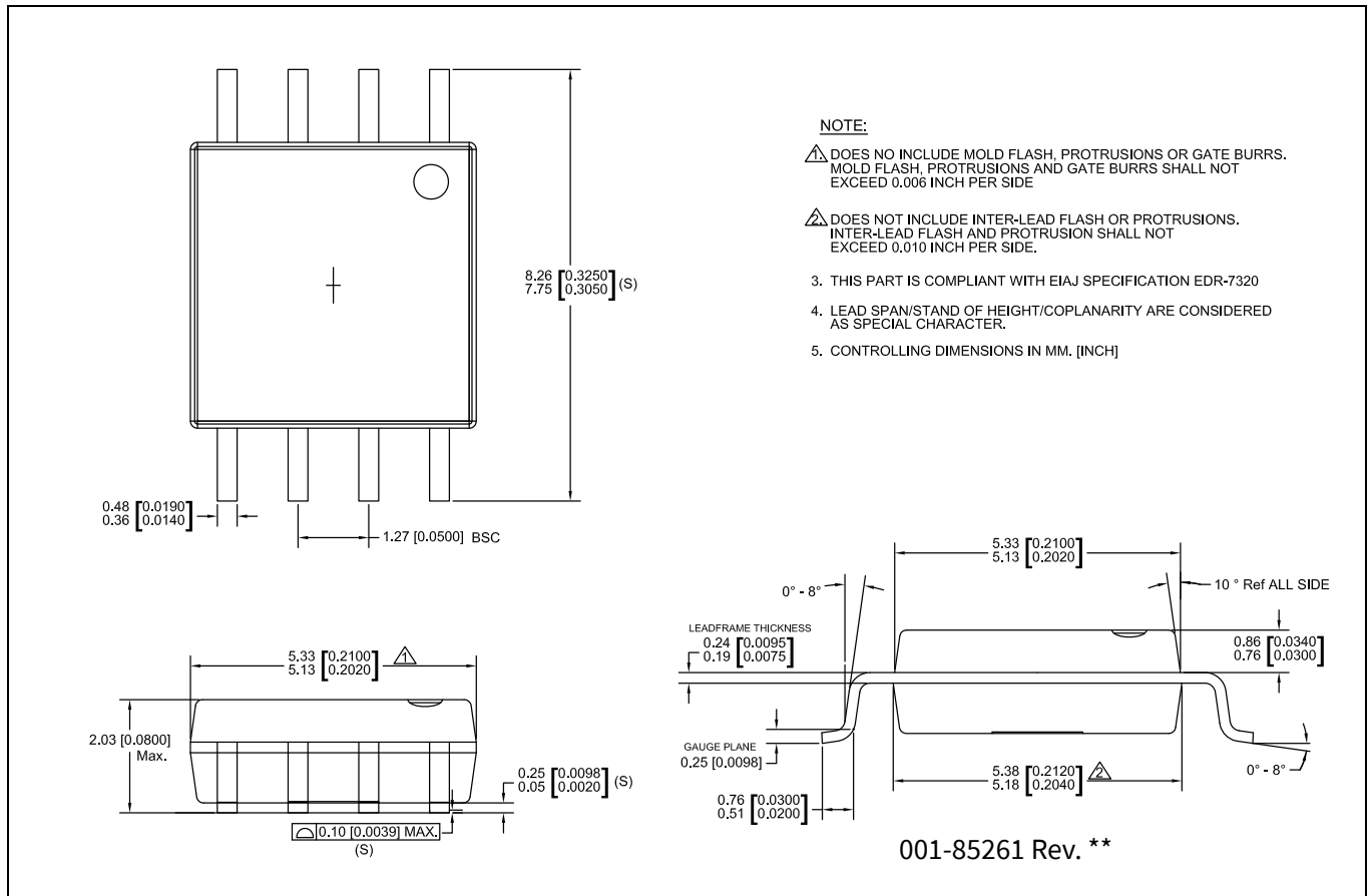
Figure 122 8-pin SOIC (208 Mils) SZ820 package outline (PG-DSO-8), 001-85261
