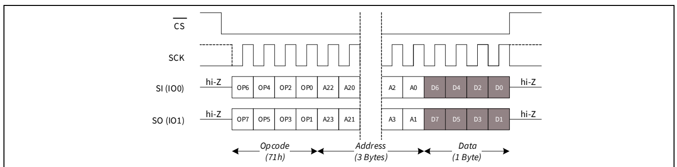
Figure 34 Write Any Register (WRAR) in DPI mode
