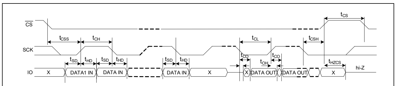
Figure 119 SPI switching timing - Multiple I/O, DDR [31]
