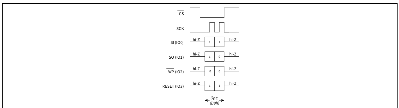
Figure 102 Deep power-down mode operation in QPI mode
