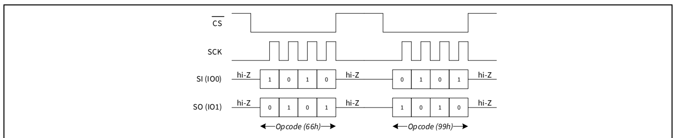
Figure 108 Software Reset timing in DPI mode
