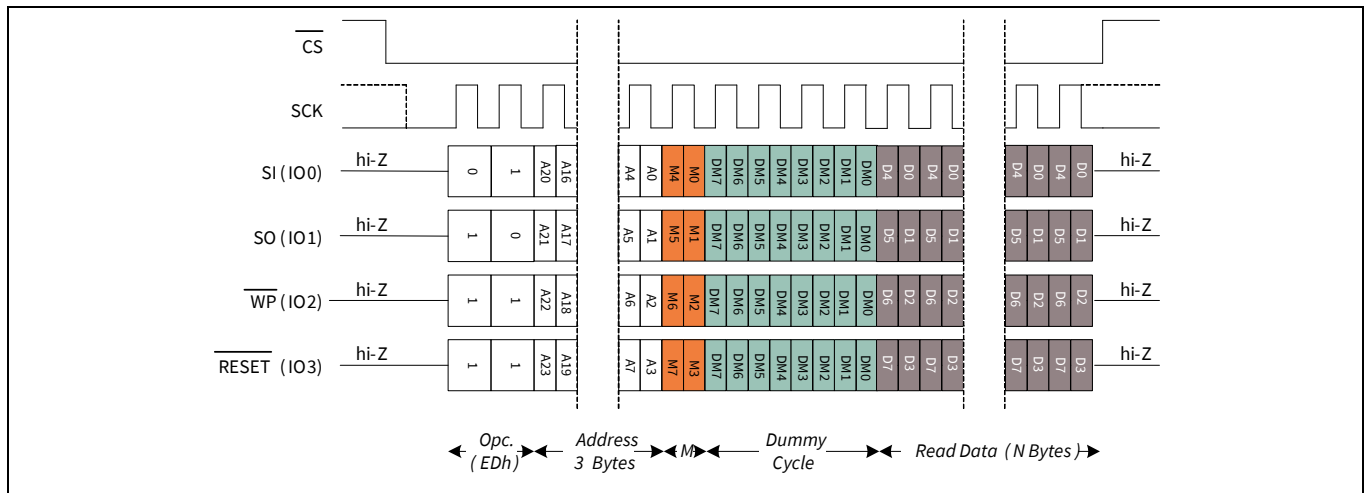
Figure 66 Quad I/O Read in DDR (DDRQIOR) – In QPI Mode
