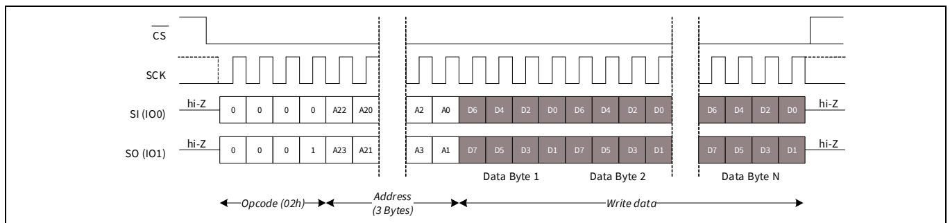
Figure 40 Memory Write (WRITE) in DPI mode
