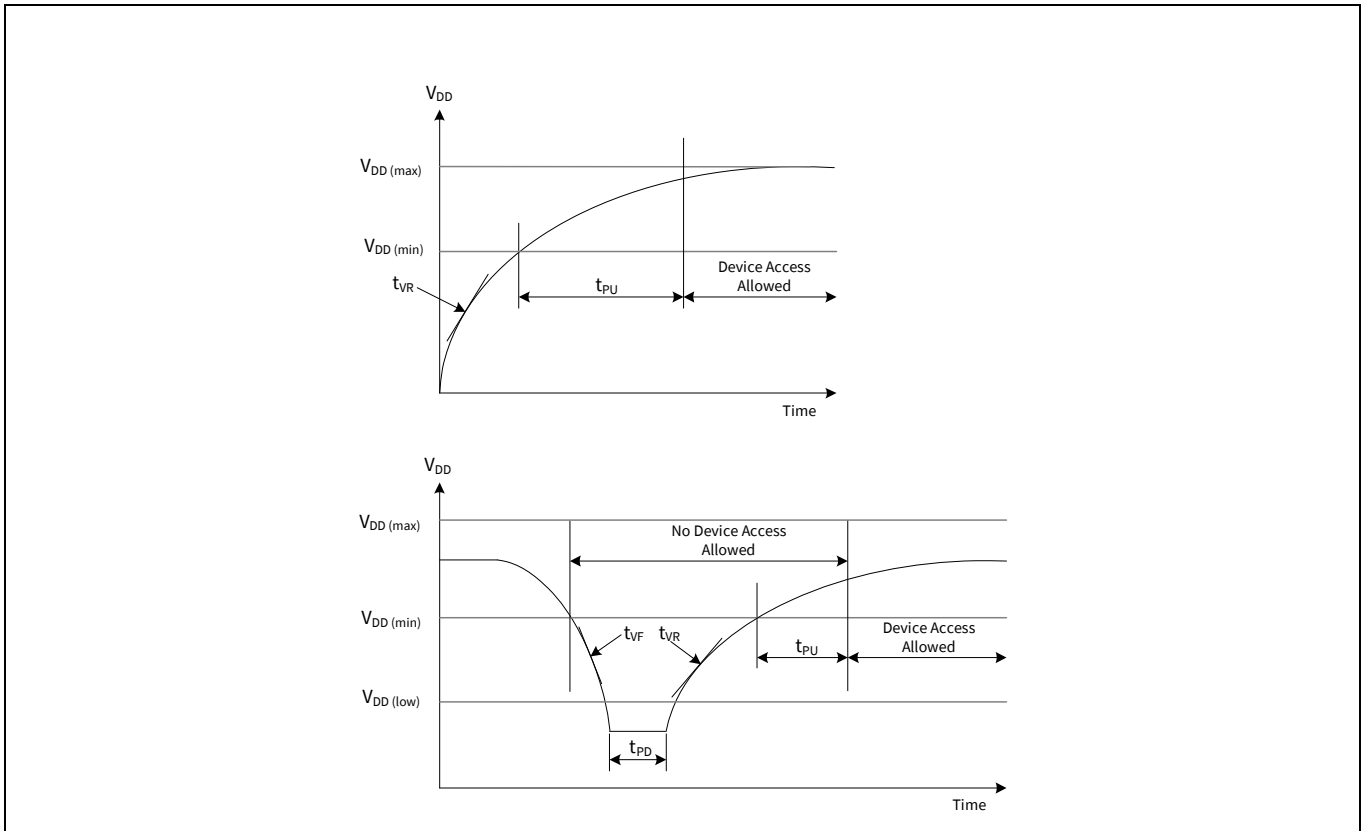
Figure 121 Power cycle timing
