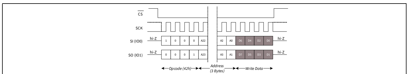
Figure 68 Special Sector Write (SSWR) in DPI Mode (WREN is not shown)
