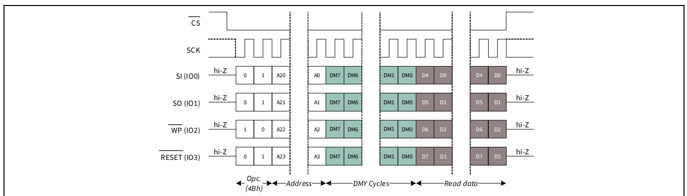
Figure 72 Special Sector Read (SSRD) in QPI mode
