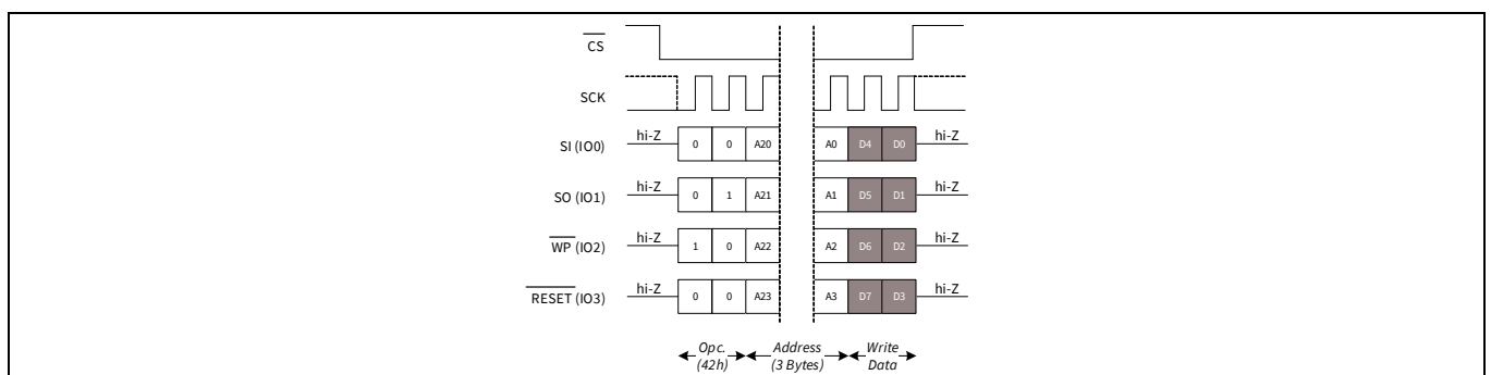
Figure 69 Special Sector Write (SSWR) in QPI Mode (WREN is not shown)
