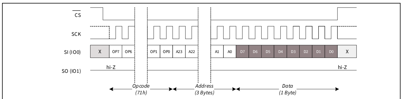
Figure 33 Write Any Register (WRAR) in SPI mode
