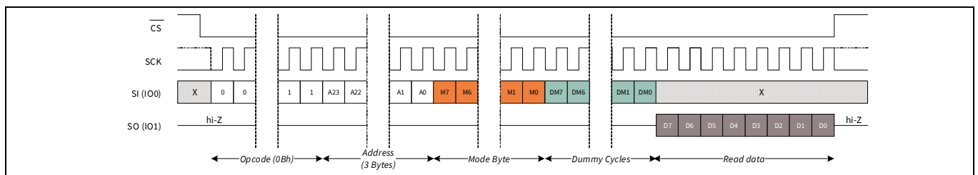
Figure 55 FAST_READ in SPI mode
