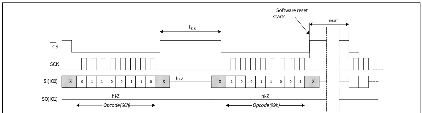
Figure 107 Software Reset timing in SPI mode
