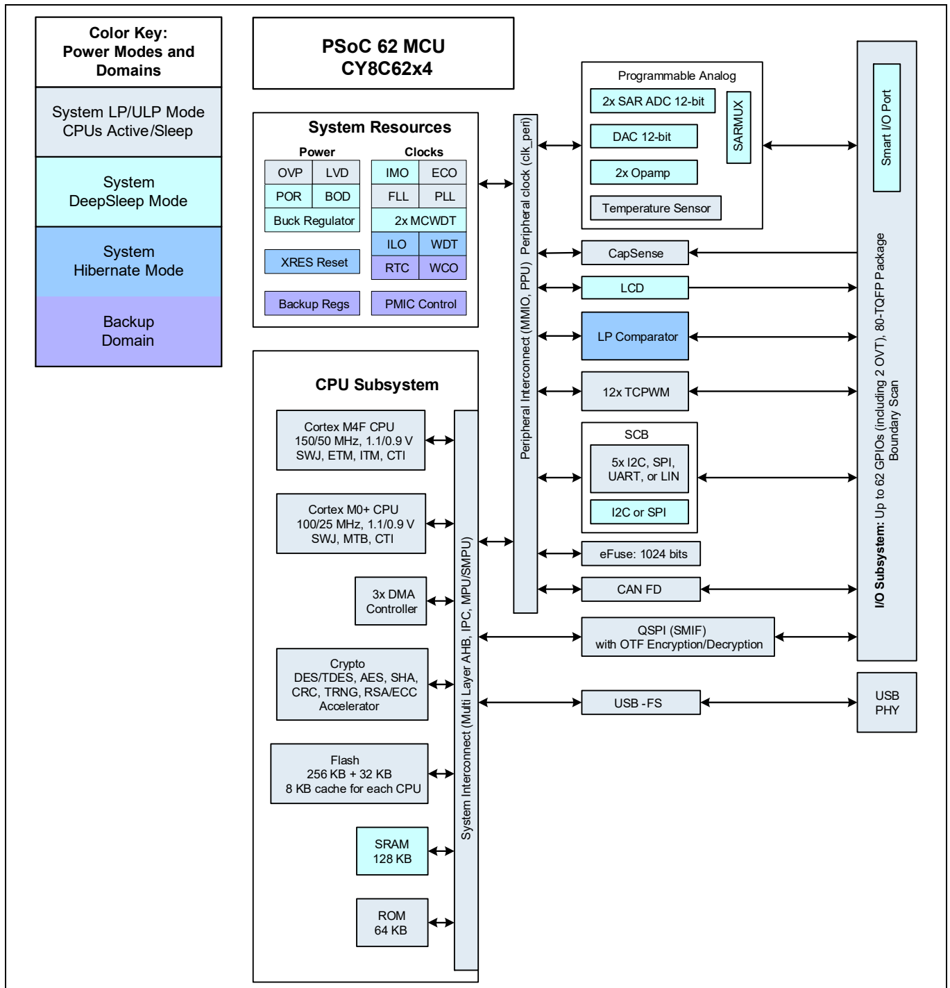
Figure 2 Block diagram
