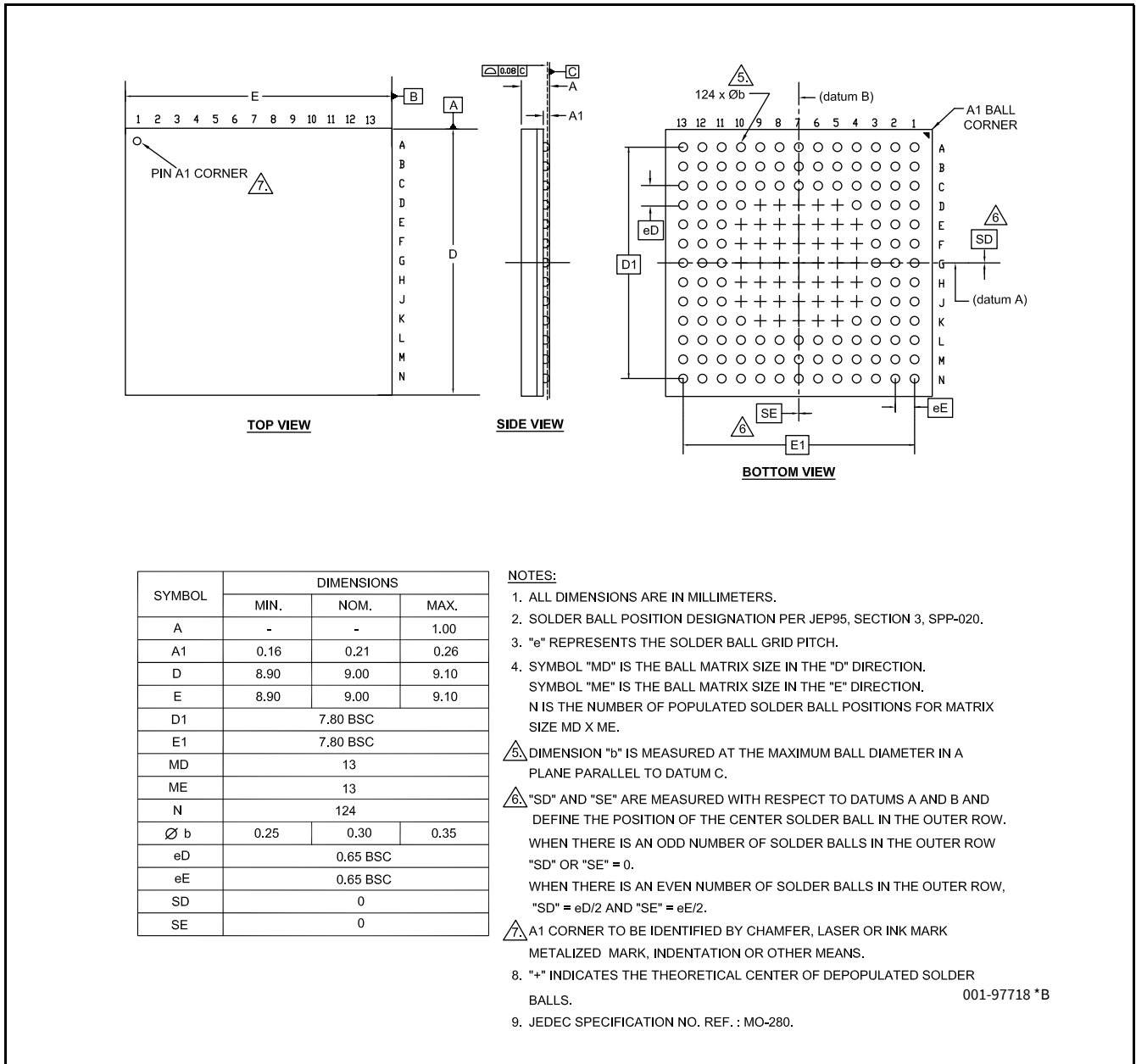
Figure 20 128-TQFP 14.0 x 20.0 x 1.4 mm, PG-VFBGA-124
