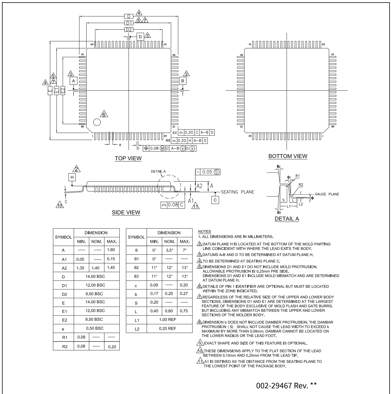
Figure 23 80-pin TQFP ((12.0 x 12.0 x 1.6 mm) AZ80A) package outline (PG-TQFP-80)
