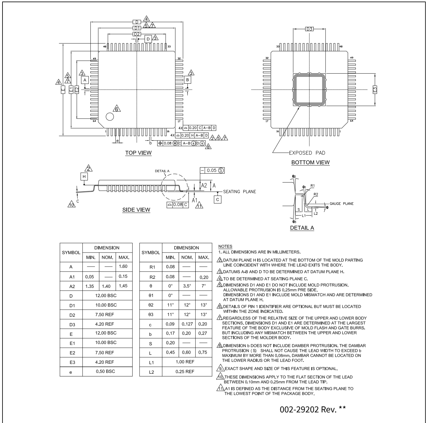
Figure 24 64-pin E-TQFP ((10.0 x 10.0 x 1.6 mm) AE64A 4.2 x 4.2 mm E-Pad package outline (PG-TQFP-64)
