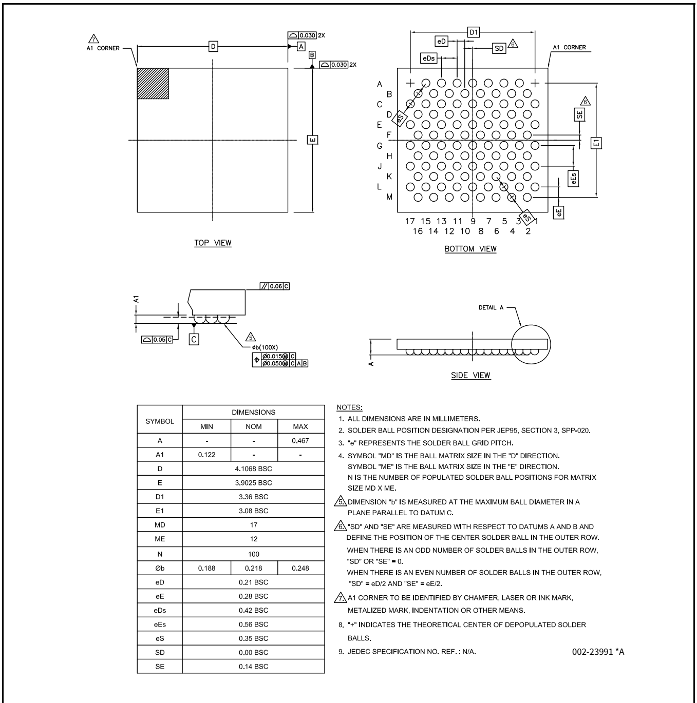
Figure 22 68-pin QFN ((8 x 8 x 1 mm) LT68D, 6.2 x 6.2 mm E-Pad (Sawn type)) package outline (PG-VQFN-68)
