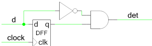
Figure 3. Falling Edge Schematic
