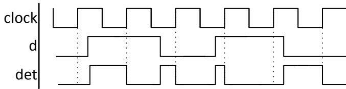
Figure 6. Either Edge Waveform
