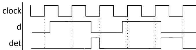
Figure 4. Falling Edge Waveform
