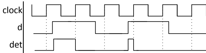
Figure 2. Rising Edge Waveform
