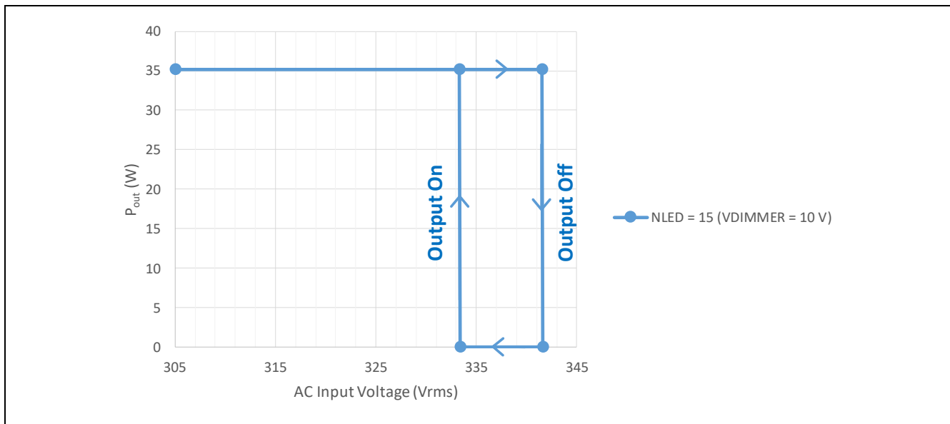
Figure 25 Input UVP and brown-out maximum power reduction
