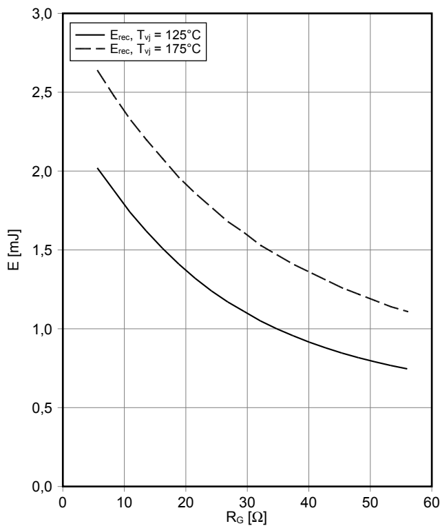
开关损耗 二极管, 逆变器 (典型) switching losses Diode, Inverter (typical) E_{rec} = f(R_G) I_F = 35 \text{ A}, V_{CE} = 600 \text{ V}
