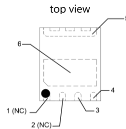
Package Outline
