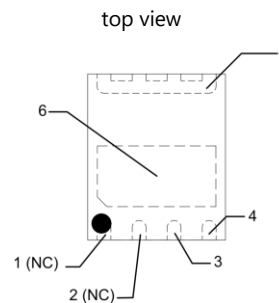
Package Outline
