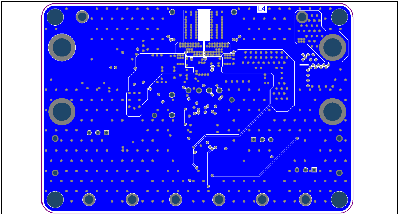
Figure 10 PCB layout bottom view
