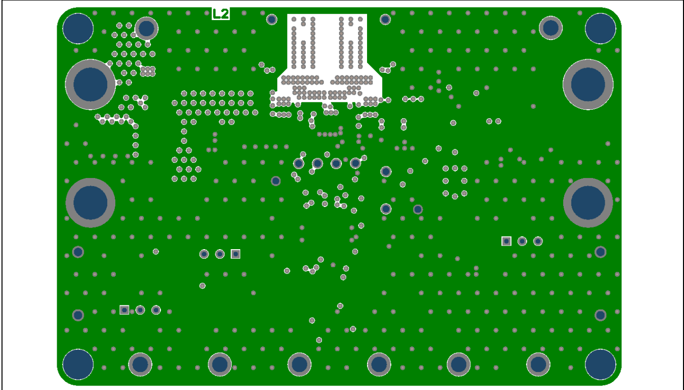
Figure 8 PCB layer 2
