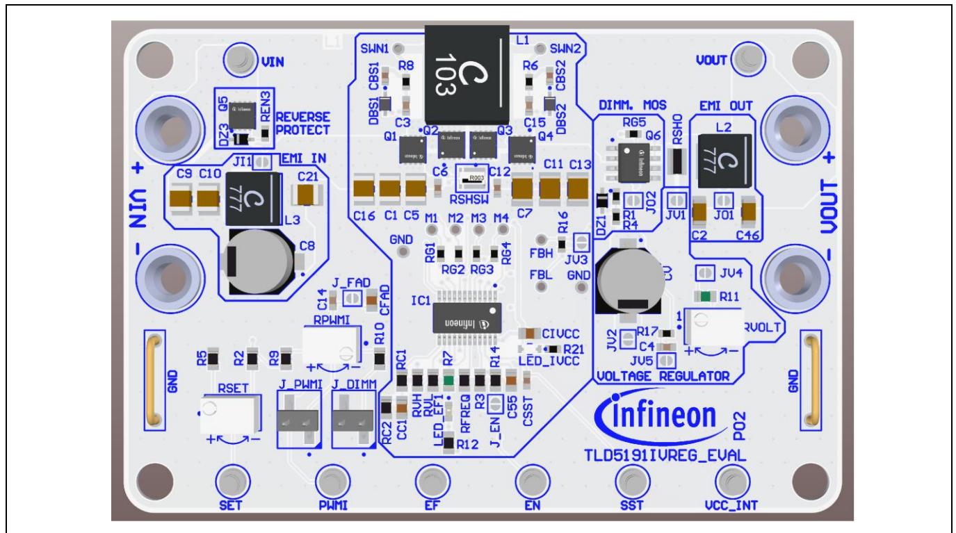
Figure 1 TLD5191IVREG-EVAL board
