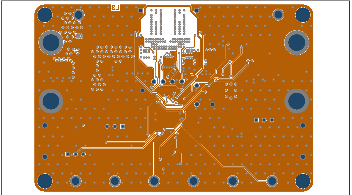
Figure 9 PCB layer 3
