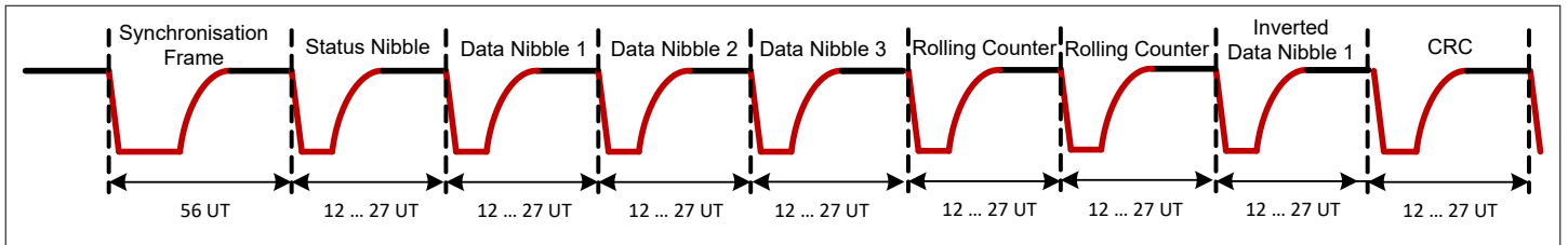
Figure 10 SENT single secure frame
