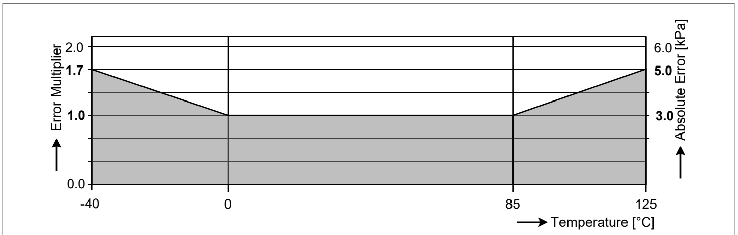
Figure 4 Accuracy for pressure acquisition
