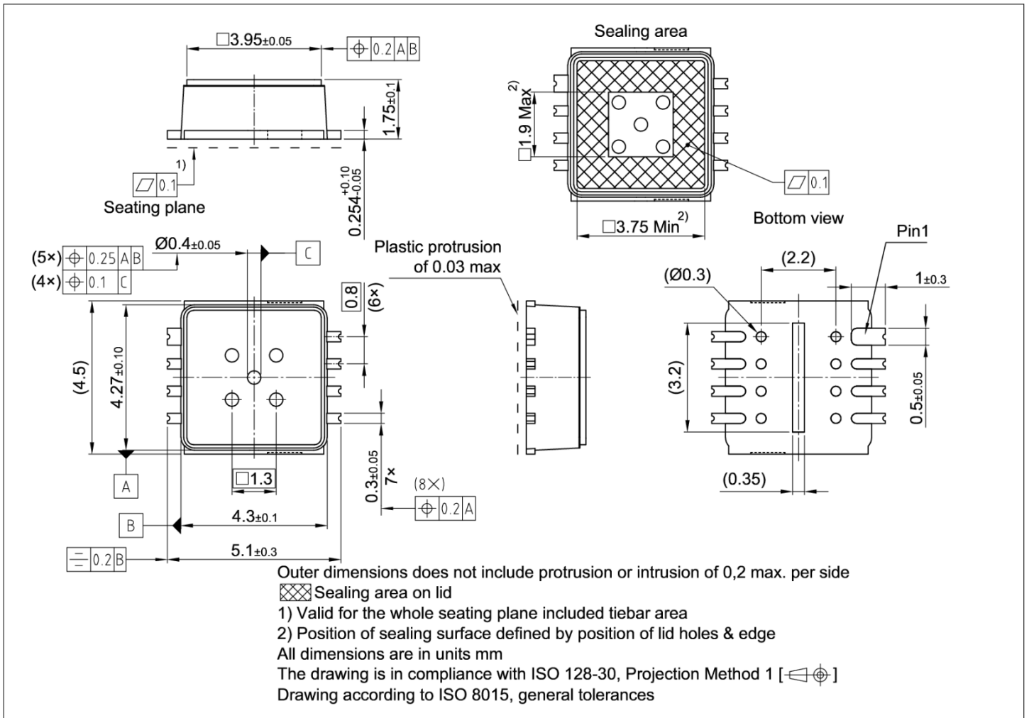
Figure 41 PG-DFN-8-1 outlines
