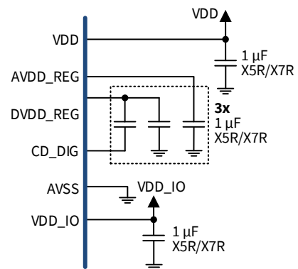
Figure 11.11: Decoupling/supply capacitor schematic with recommended specifications
