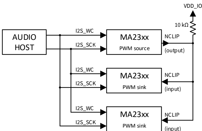
Figure 11.23: PWM synchronization for multiple MA2306PNS devices
