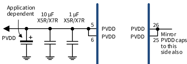
Figure 11.14: Typical decoupling for multi-layer ceramic capacitors (MLCC) with different package sizes
