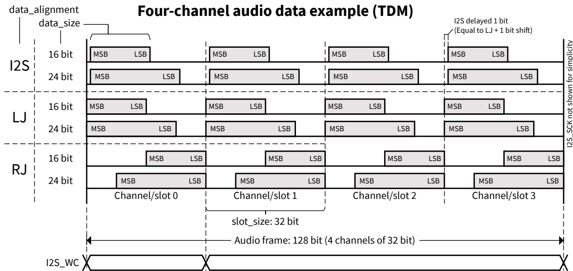
Figure 11.17: Audio data configuration/timing for four channels. Note that choosing 'I2S' in data_alignment for MA2306PNS does not restrict the data stream to only two channels. 'I2S' in data_alignment just refers to the data being aligned to the left and delayed by one bit.
