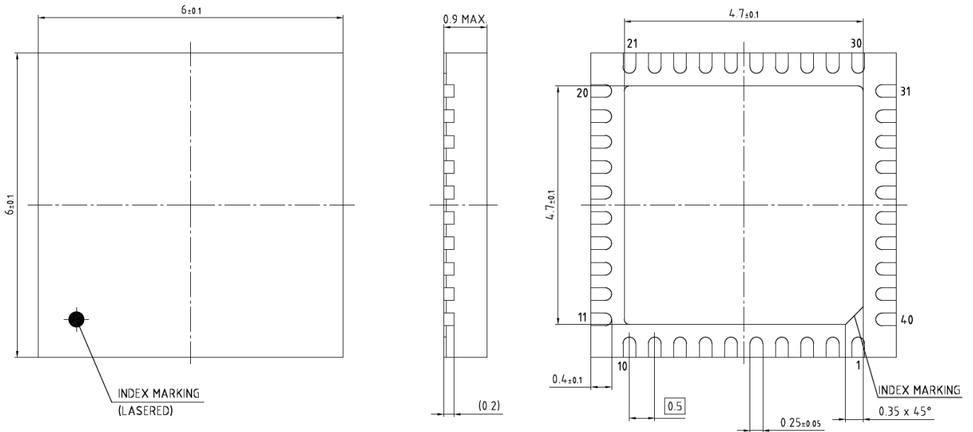
Figure 16.1: QFN pad-down 40-pin MA2306PNS package dimensions. Left: Top view. Middle: Side view. Right: Bottom view.
