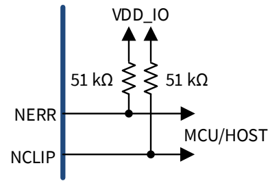
Figure 11.8: NERR/NCLIP schematic
