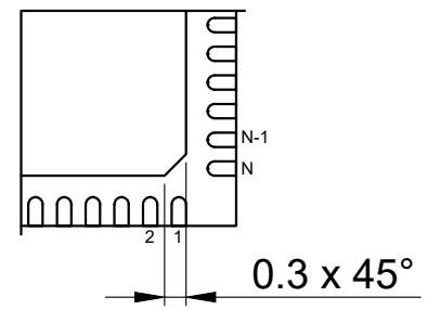
Detail "C" option 2
