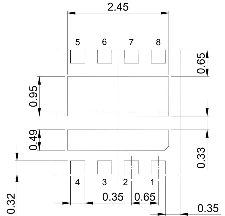
Bottom view
