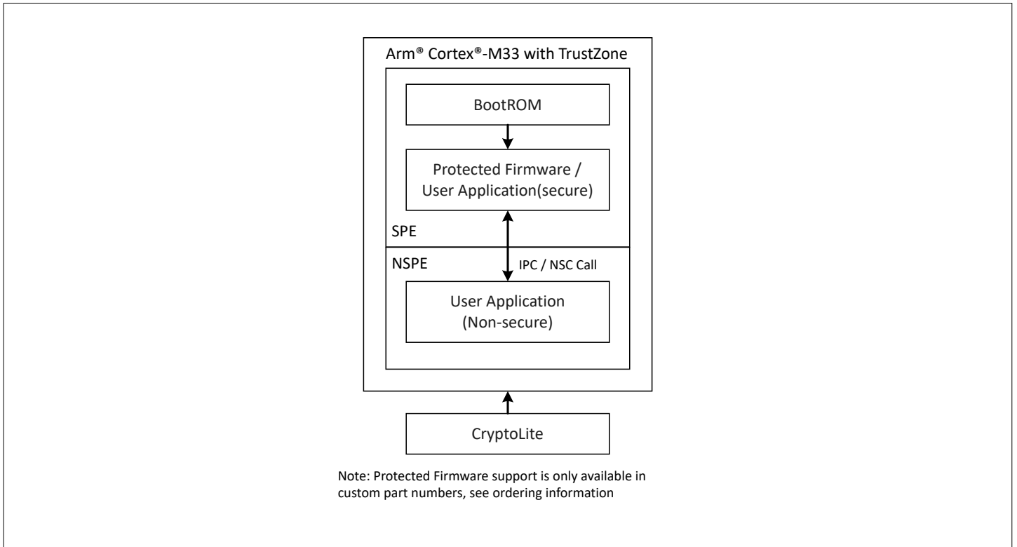
Figure 6 Security architecture diagram
