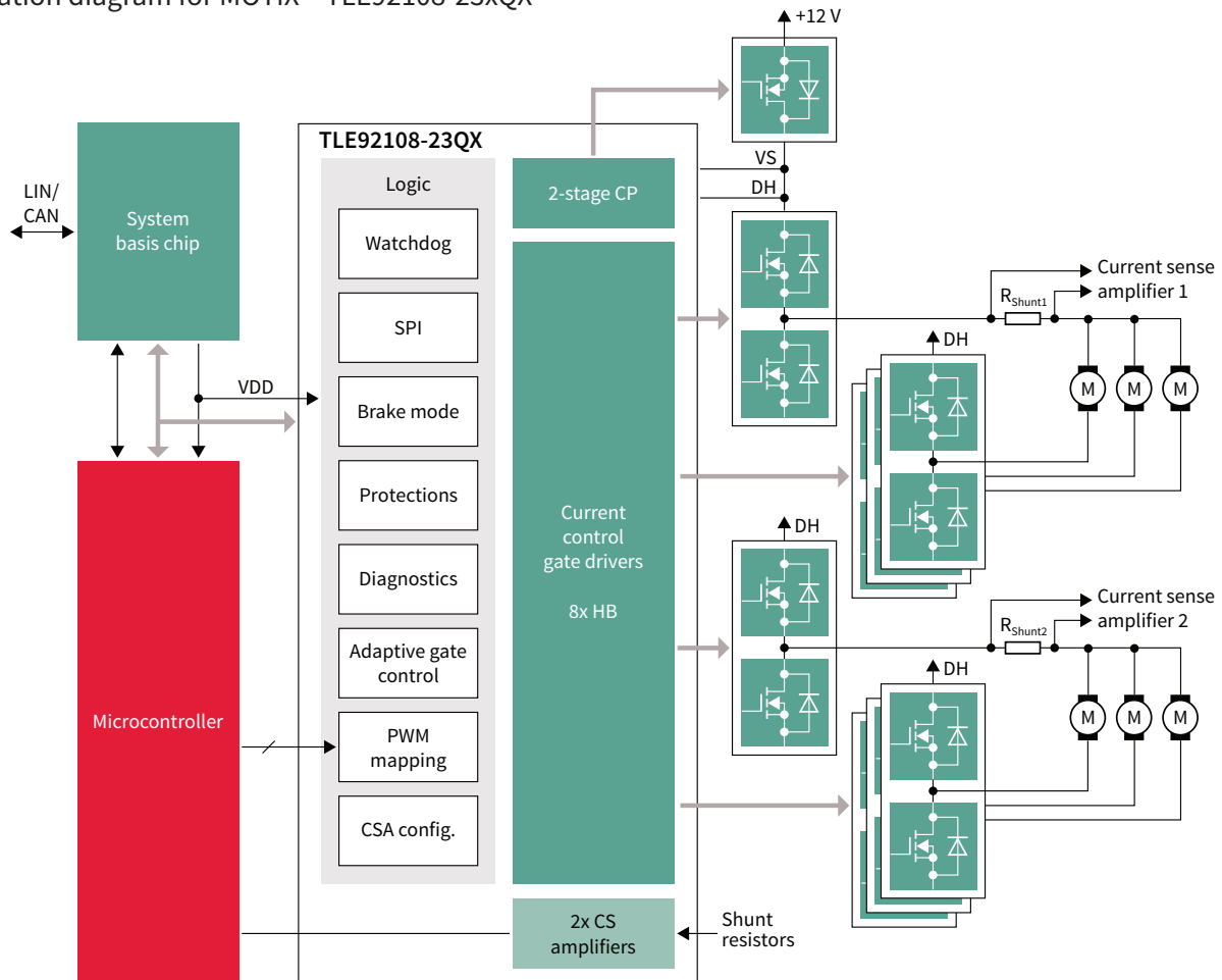
Application diagram for MOTIX™ TLE92108-23xQX
