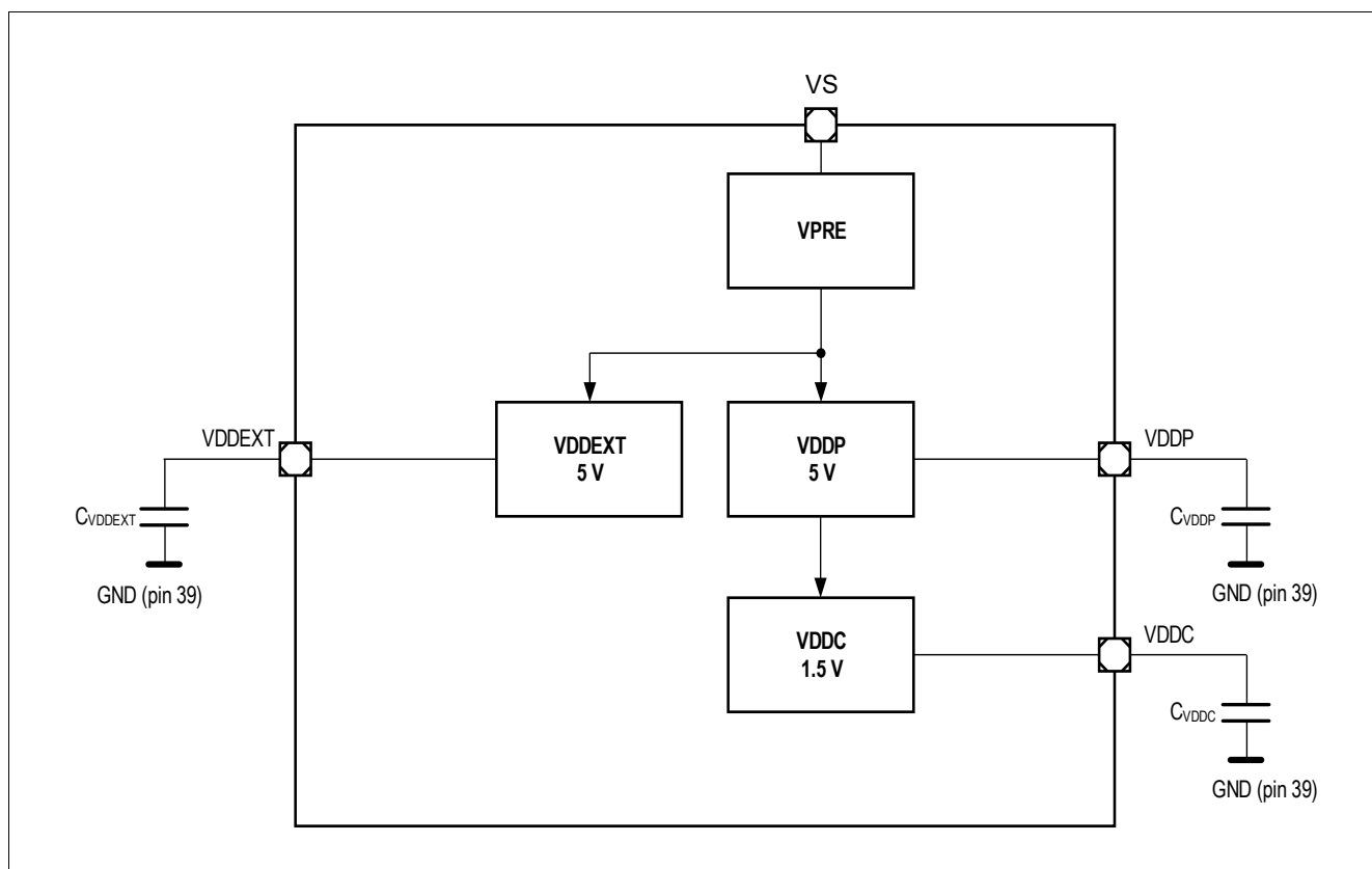
Figure 34 Load-sharing scenario for the VPRE regulator
