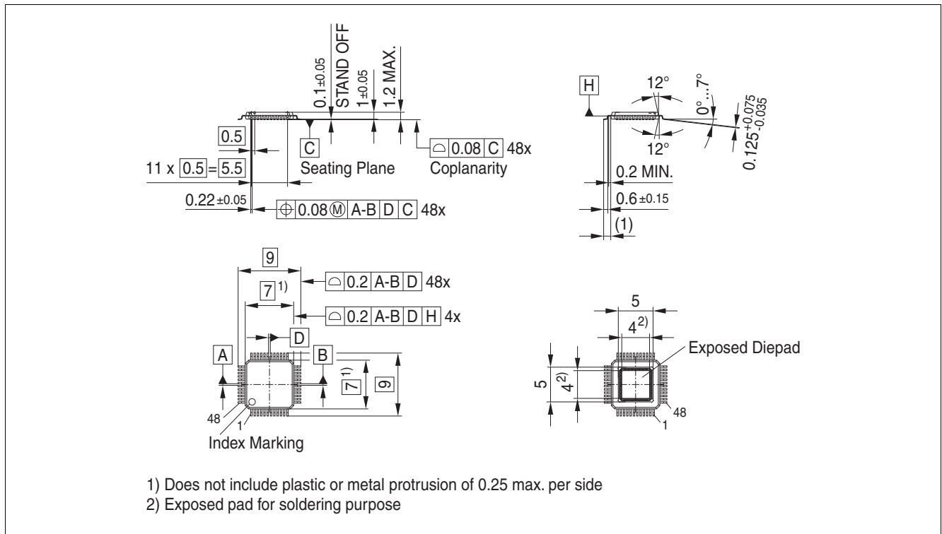
Figure 39 Package outline TQFP-48-10 1)
