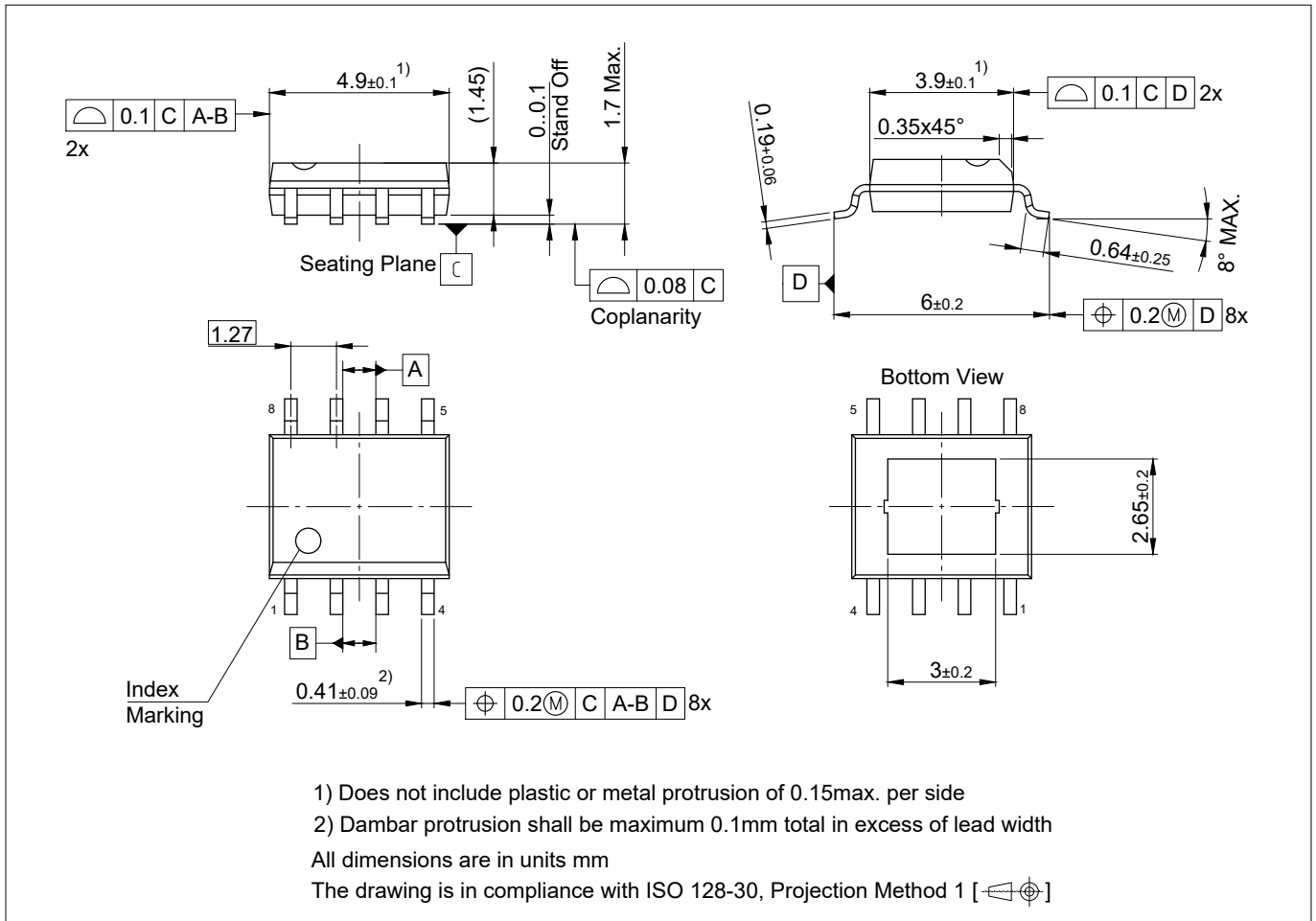
Figure 4 PG-DSO-8
