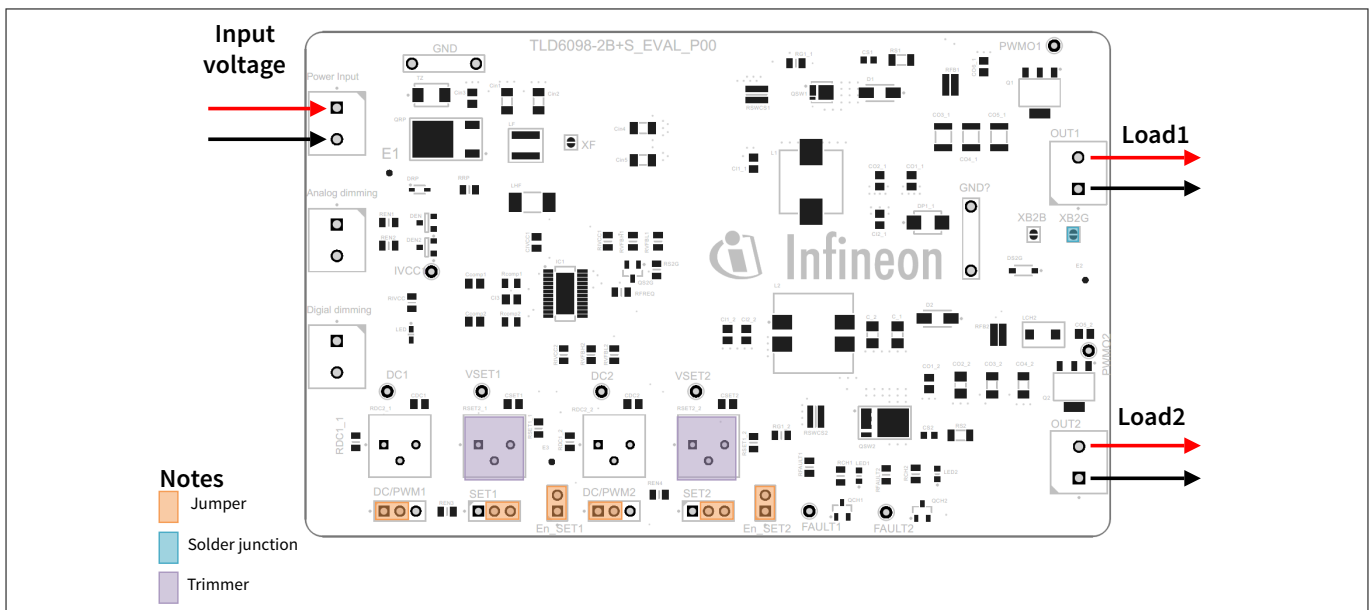
Figure 3 Current adjustment
